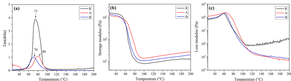
Fig. 7. DMA analysis of tested adhesives R, A and B represented as: (a) \tan(\delta) , (b) storage modulus, G' and (c) loss modulus, G''
