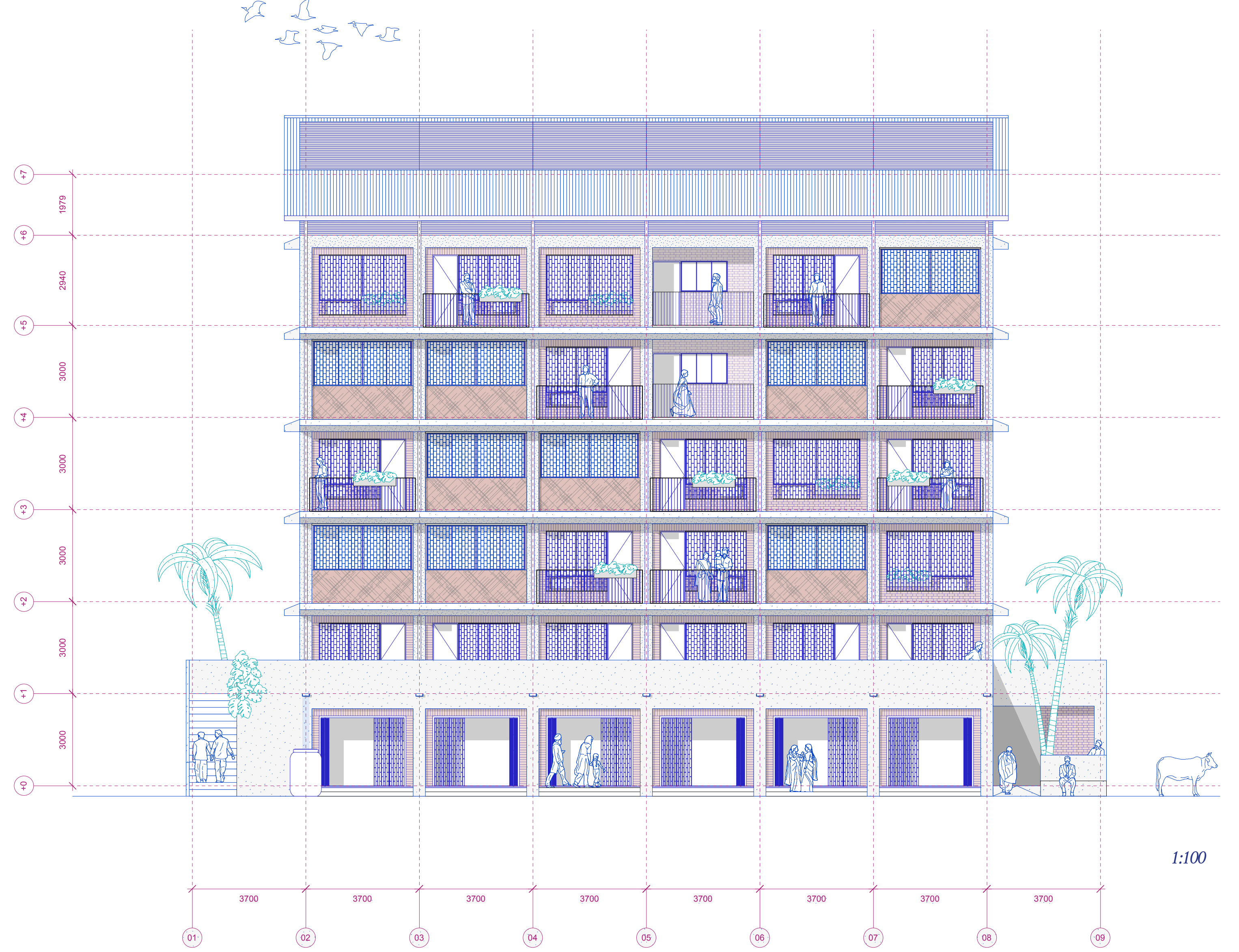
ELEVATIONS East
