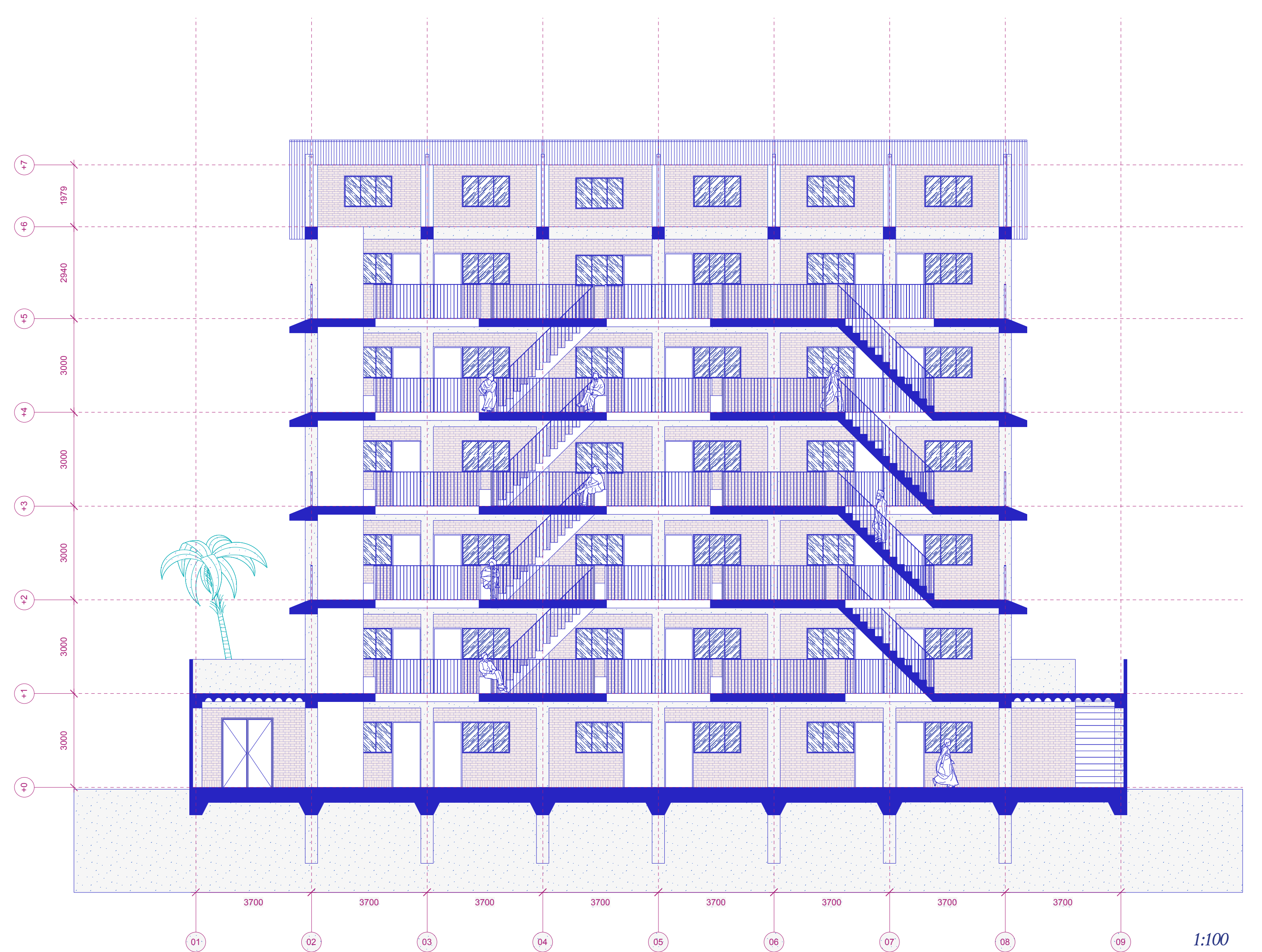
SECTIONS S-N
