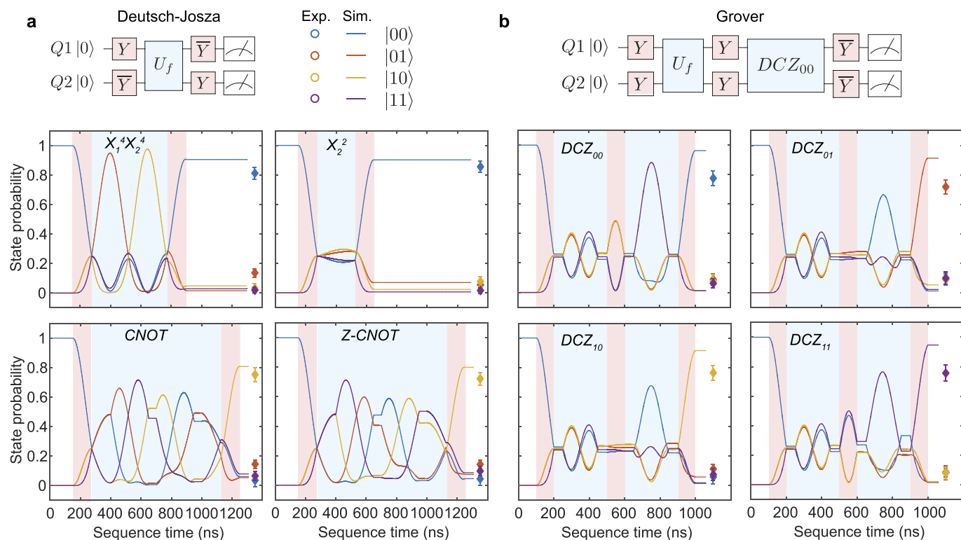
Extended Data Figure 10 | Simulation of the Deutsch-Josza and Grover search algorithms using the DCZ gate. a, b , Two-spin probabilities as a function of the sequence time during the Deutsch-Josza algorithm ( a ) and the Grover search algorithm ( b ) for each function, using the decoupled
