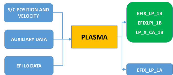
Figure 2. Schema of the L1B PLASMA operational processor. The blue boxes on the left side represent the input files, the central yellow box represents the PLASMA processor, and the right-side boxes represent the processor outputs. In particular, the green box contains the EFI-LP L1B data products.
