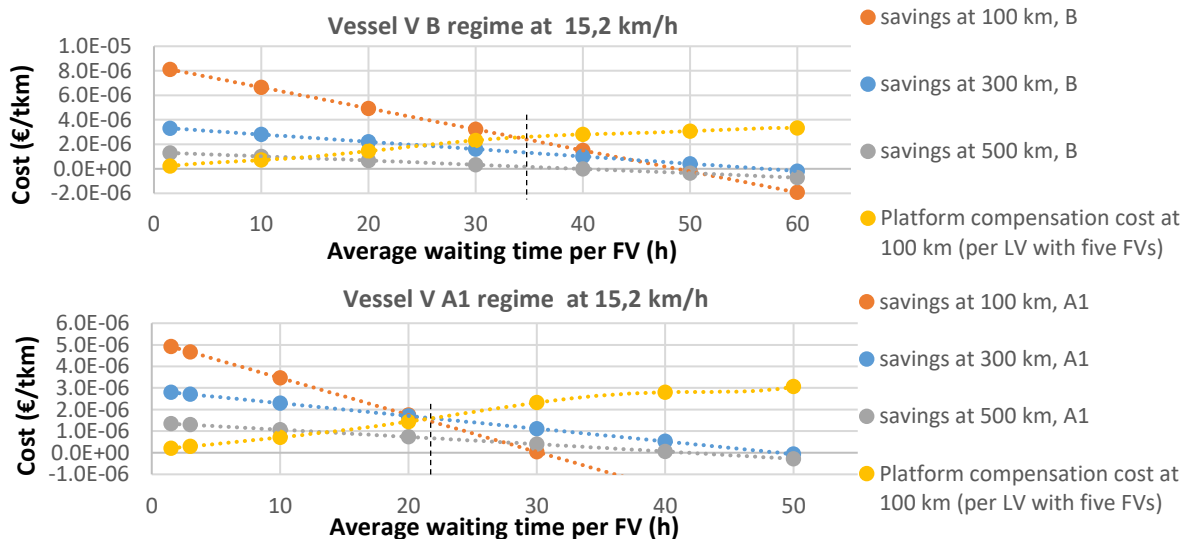
Figure 52: Waiting Time Variation for Vessel Class V
