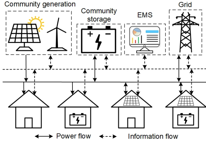
Figure 3.2: A physical ICES system
