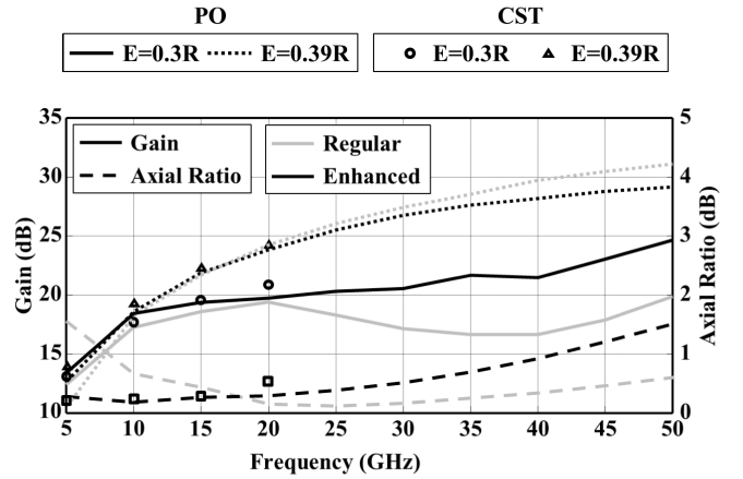
Fig. 16. Simulated broadside gain and axial ratio of the secondary fields for the regular and the enhanced structures using the hyperhemispherical and the elliptical extension. The gain takes into account of losses due to matching, reflection, polarization, and front-to-back ratio.
