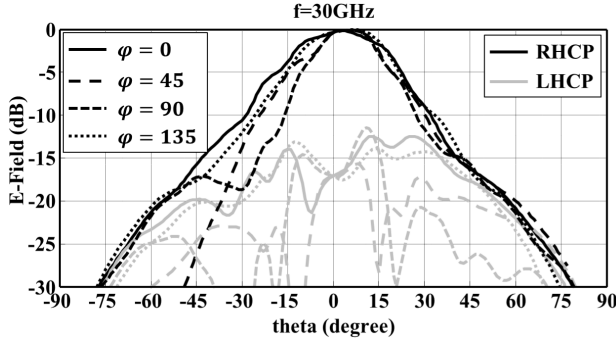
Fig. 11. Simulated radiation patterns of the enhanced logarithmic spiral antenna ( \delta = 45^\circ ) fed by a microstrip on different \varphi planes at the frequency 30GHz.
