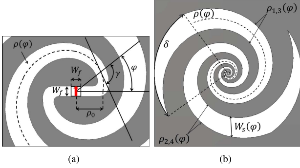
Fig. 2. Logarithmic spiral antenna. (a) Antenna geometry. (b) Design parameters.
