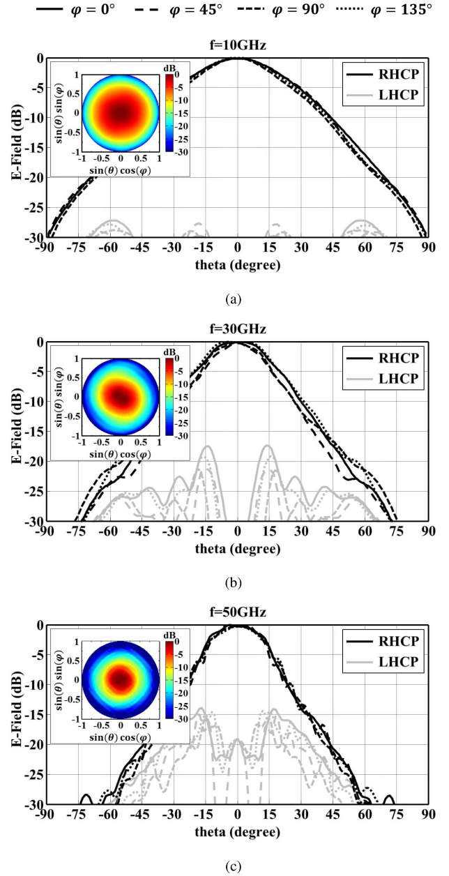
Fig. 9. Simulated radiation patterns (primary fields) of the enhanced logarithmic spiral antenna ( \delta = 45^\circ ) inside the dielectric on different \varphi planes at the frequencies (a) 10GHz, (b) 30GHz and (c) 50GHz. Insets: 2-D radiation patterns of the RHCP component.
