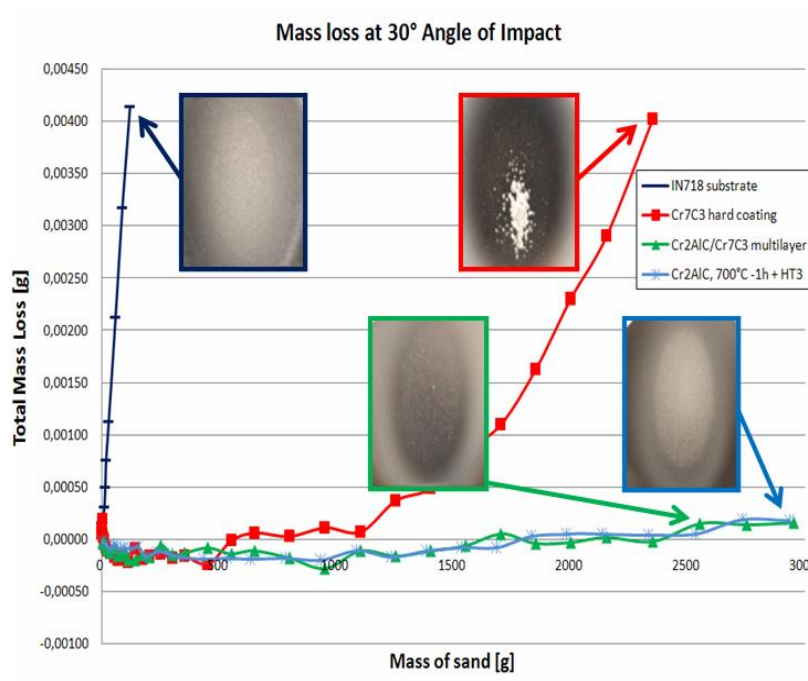
Figure 1.2 Mass loss of IN718 uncoated (dark blue) and coated with \text{Cr}_7\text{C}_3 (red), \text{Cr}_2\text{AlC}/\text{Cr}_7\text{C}_3 multilayers (green) and \text{Cr}_2\text{AlC} (blue).
