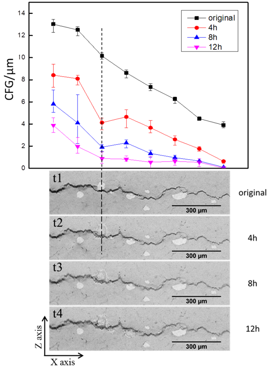
Figure 5.8 (Top) Crack face gap (CFG) calculated along the crack growth direction for different healing times; (below) 2D X-ray tomographic cross sections correlated to the CFG plots at different healing stages. The dashed line indicates the large CFG decrease near surface breaking Cr particle.
