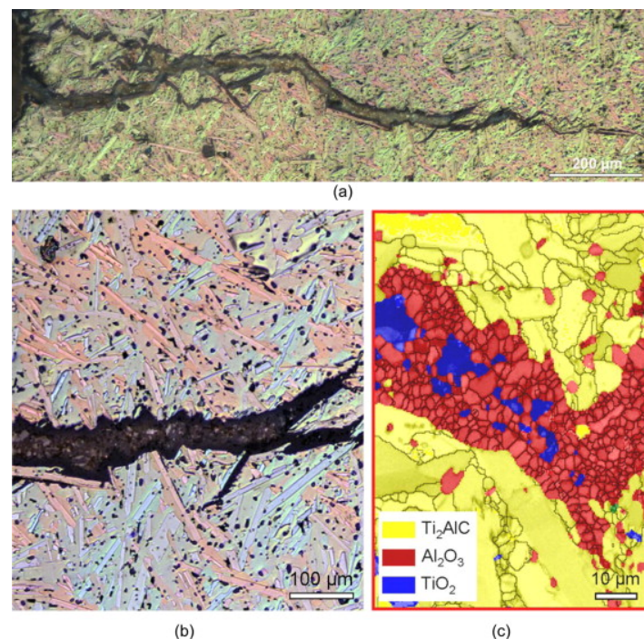
Figure 1.3 (a) Low magnification optical image of 3 point bending test induced cracks healed in air at 1200 °C for 100h; (b) Enlarged optical image taken from (a); (c) EBSD phase map of a detail of the healed damage zone. After [13]
