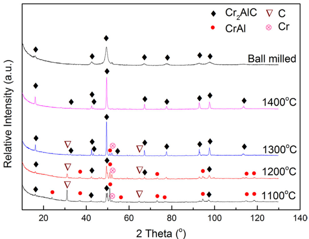
Figure 2.1 X-ray diffractograms of a Cr-Al-C powder mixture pressure-less sintered at different temperatures, including a ball-milled powder of the material sintered at 1400 °C.
