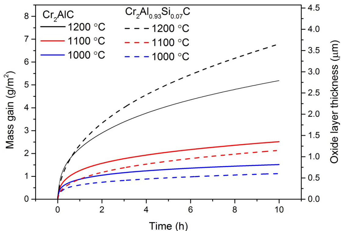
Figure 3.4 Mass change due to oxidation of \text{Cr}_2\text{AlC} (solid lines), and \text{Cr}_2\text{Al}_{0.93}\text{Si}_{0.07}\text{C} (dashed lines) at 1000, 1100 and 1200 °C in dry synthetic air for 10 h. Both mass gain and equivalent oxide layer thickness as a function of oxidation time were plot on left and right axes, respectively.
