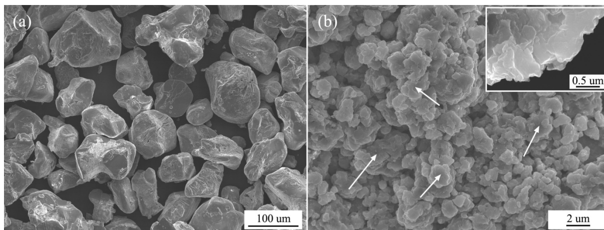
Figure 2.2 SEM images of the milled pressure-less sintered Cr 2 AlC at 1400 °C. (a) coarse-grained and (b) fine-grained. The arrows indicate flake like shape and the insert shows the plate like morphology at the edge.
