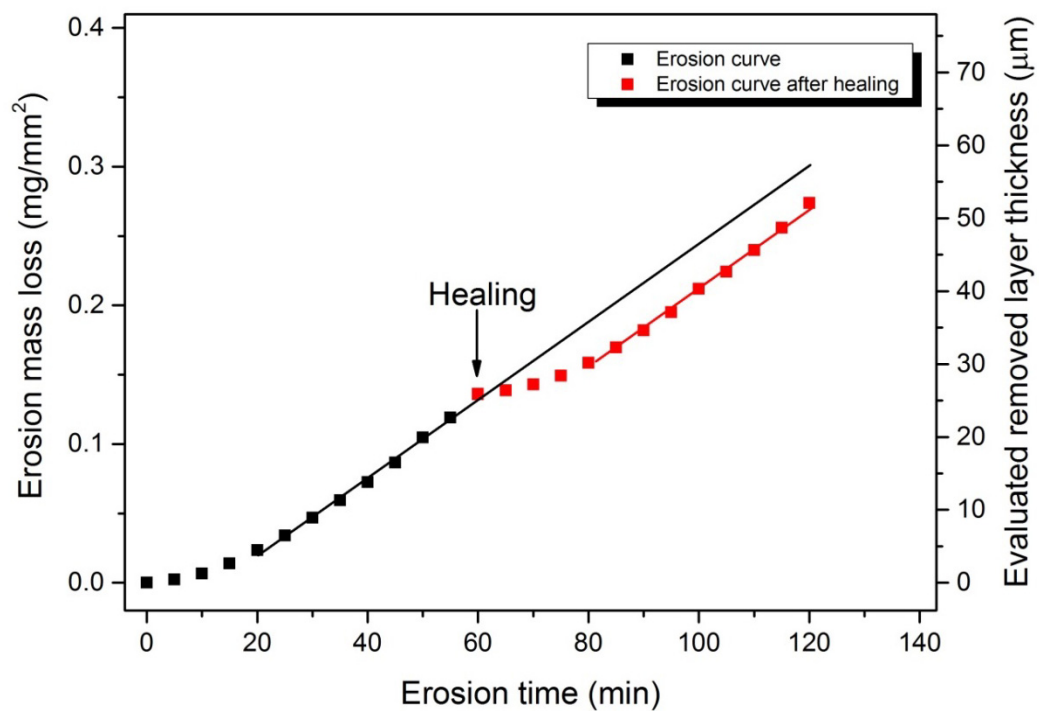
Figure 6.4 Erosion mass loss and evaluated removed layer thickness as a function of erosion time of the \text{Cr}_2\text{AlC} virgin material (black dots) and the healed material (red dots). The black and red solid straight lines represent the steady state erosion of the virgin and healed material, respectively. The steady state erosion is extrapolated to compare with the erosion of the healed material. Erosion by 2 g/min spherical glass beads having an average diameter of 95 \mu\text{m} and 110 m/s impact velocity. Healing of impact crack damage at 1200 ^\circ\text{C} for 10 minutes in air.
