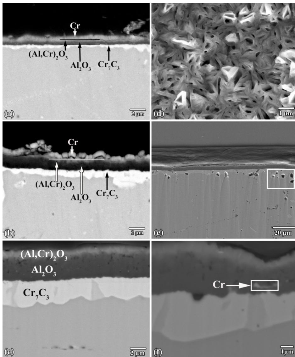
Figure 3.6 BSE images of cross section of \text{Cr}_2\text{Al}_{(0.93)}\text{Si}_{(0.07)}\text{C} after isothermal oxidation for 10 h in dry synthetic air at (a) 1000, (b) 1100, (c) 1200 °C, (d) is a SEM image of surface morphology and (e), (f) are BSE images of cross section of \text{Cr}_2\text{Al}_{(0.93)}\text{Si}_{(0.07)}\text{C} with different magnifications after oxidation at 1200 °C for 10 h in dry synthetic air.
