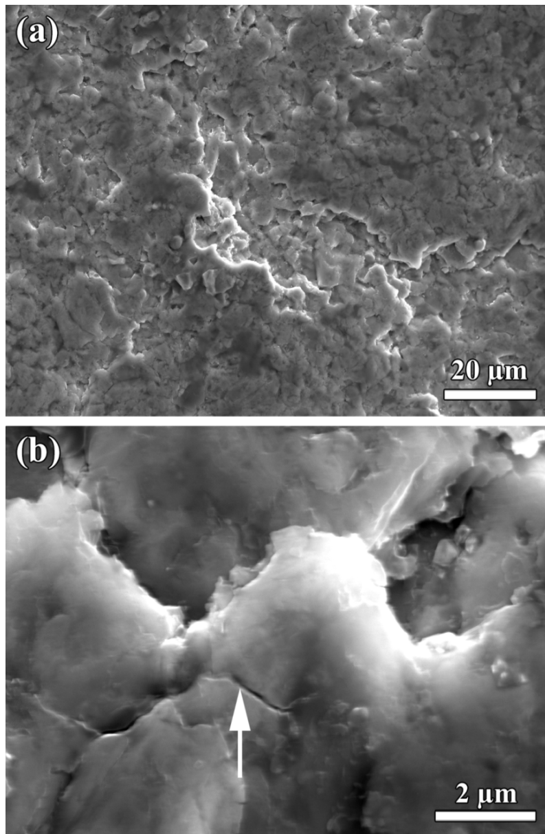
Figure 6.2 SEM images of the surface after 60 minutes erosion with 2 g/min spherical glass beads having an average diameter of 95 μm and 110 m/s impact velocity: (a) with low and (b) high magnification. The arrow indicates a crack.
