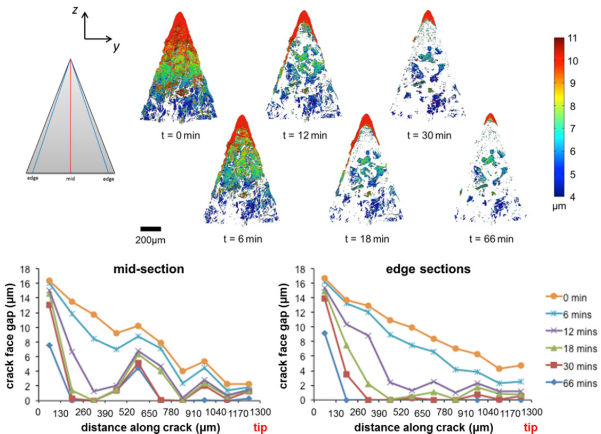
Figure 4.4 Planar views of the 3D datasets segmented to show the second crack in Ti_2AlC both initially and at different stages of healing at 1500 K in air. This second crack (cf. Figure 4.2) has a length of 1.3 mm. The superimposed colour map represents the crack face gap (CFG). The direction of crack growth is from top (mouth) to bottom (crack-tip) in the images. The graphs show the remaining opening of the crack having a length of 1.3 mm as a function of healing time for virtual sections in the middle and towards the edges of the crack (averaged over both edge trajectories).
