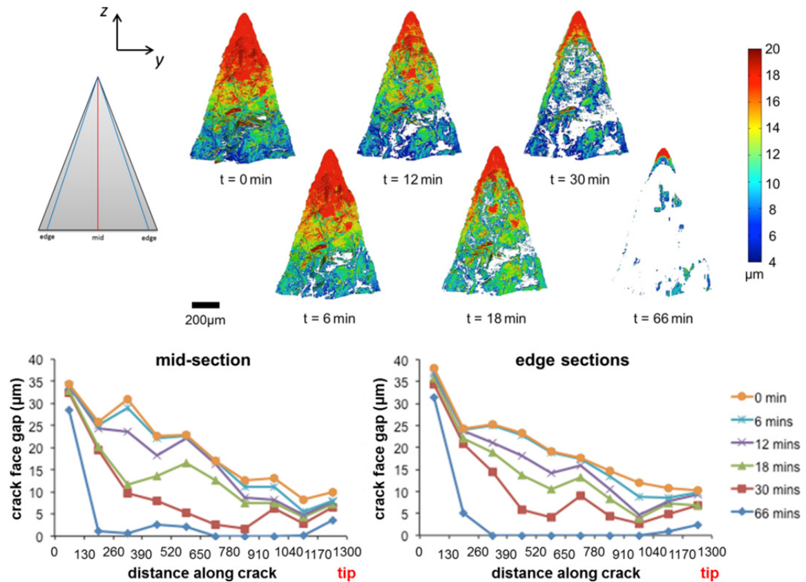
Figure 4.5 Planar views of the 3D datasets segmented to show the third, re-cracked healed second, crack in Ti_2AlC both initially and at different stages of healing at 1500 K in air. This third, re-cracked healed second crack (cf. Figure 4.2), has a length of 1.3 mm. The superimposed colour map represents the crack face gap (CFG). The direction of crack growth is from top (mouth) to bottom (crack-tip) in the images. The graphs show the remaining opening of the crack having a length of 1.3 mm as a function of healing time for virtual sections in the middle and towards the edges of the crack (averaged over both edge trajectories).
