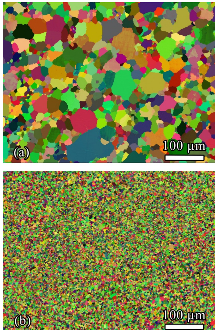
Figure 2.5 Orientation image (Euler map) of SPS sintered \text{Cr}_2\text{AlC} bulk ceramics with (a) coarse and (b) fine grains.
