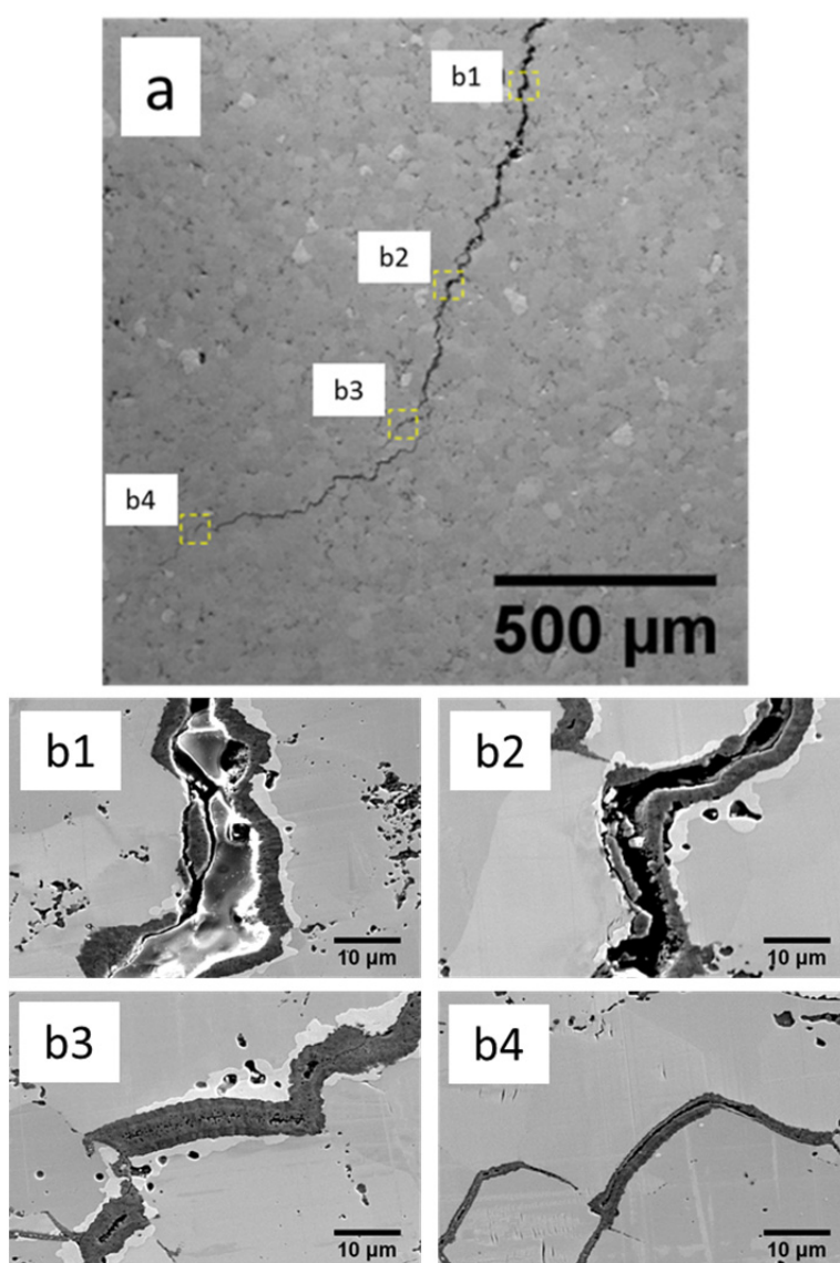
Figure 5.6 Cross sectional secondary electron SEM images of a crack after healing at 1200\text{ }^\circ\text{C} for 4 hours in air: (a) a cross section image parallel to the crack growth direction of the healed crack at low magnification; (b) higher magnification images for the areas of “b1”, “b2”, “b3”, “b4” in Figure 5.6 (a).
