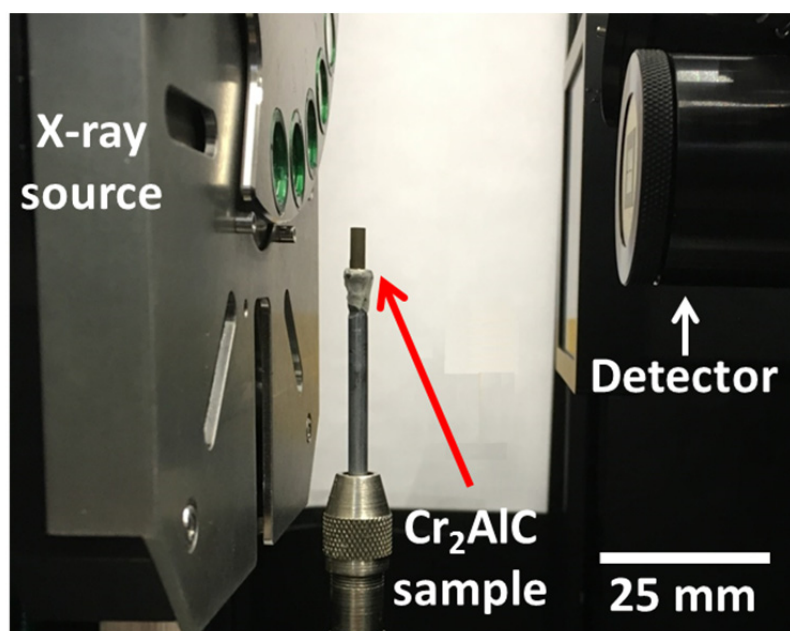
Figure 5.1 Photograph showing the set-up of the X-ray tomography experiment.
