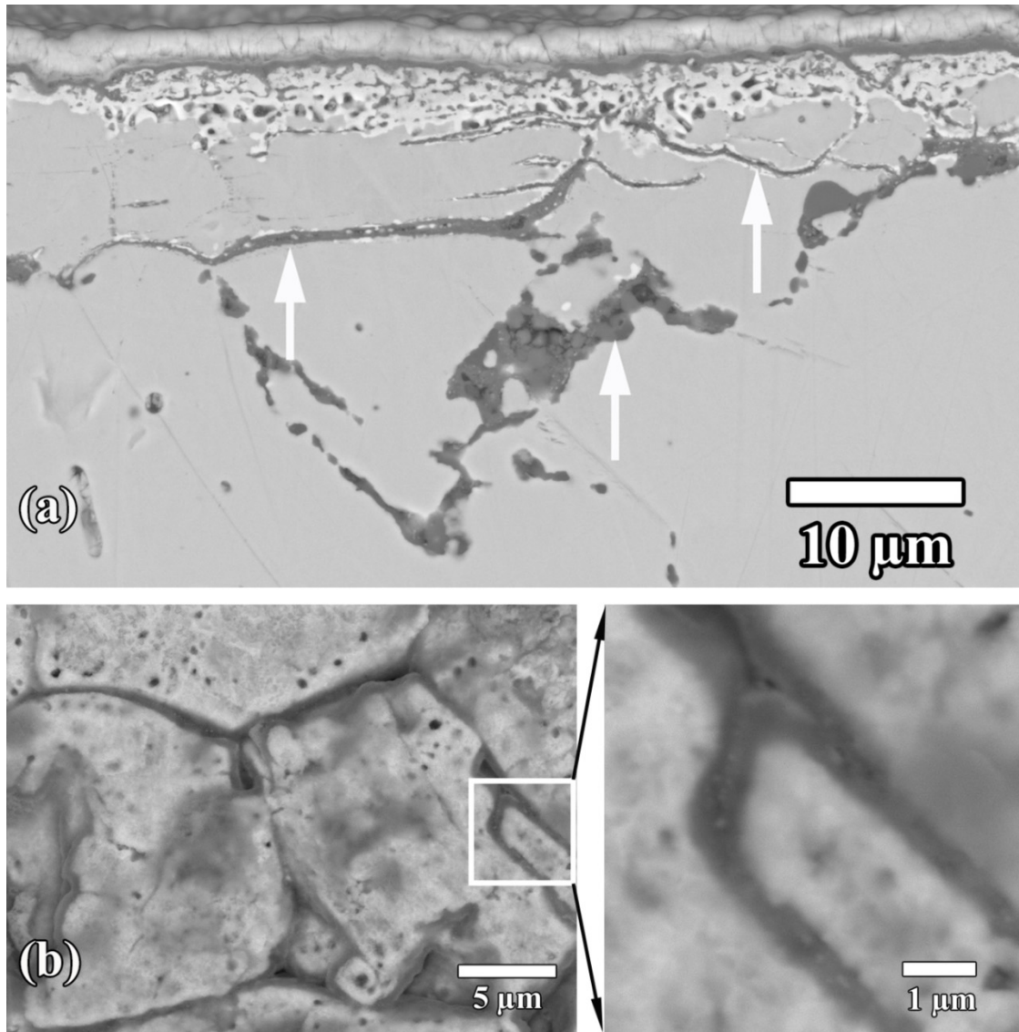
Figure 7.8 BSE images of eroded coarse-grained \text{Cr}_2\text{AlC} after healing at 1200 °C in air for 10 min. (a) Cross section with a Cr layer deposited on the surface for sample preparation. The arrows indicated the filled crack gaps and pores with \text{Al}_2\text{O}_3 (b) Top view with an enlarged section. The surface was sputtered with Ar-ions to remove the surface oxide and reveal the healed cracks.
