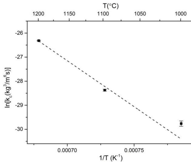
Figure 3.5 Arrhenius plot of the cubic growth rate constant of the oxide scale on \text{Cr}_2\text{AlC} .
