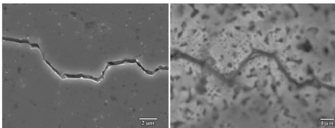
Figure 8.7.(a) Crack damage in fine grained \text{Cr}_2\text{AlC} generated by Vickers indentation; (b) Crack healed by \text{Al}_2\text{O}_3 formed in combustion environment for 4 hours.
