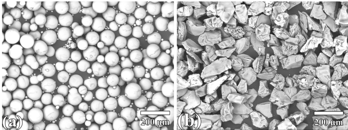
Figure 7.1 BSE images of (a) spherical micro glass beads and (b) angular corundum particles with an average diameter of 100 \mu\text{m} .
