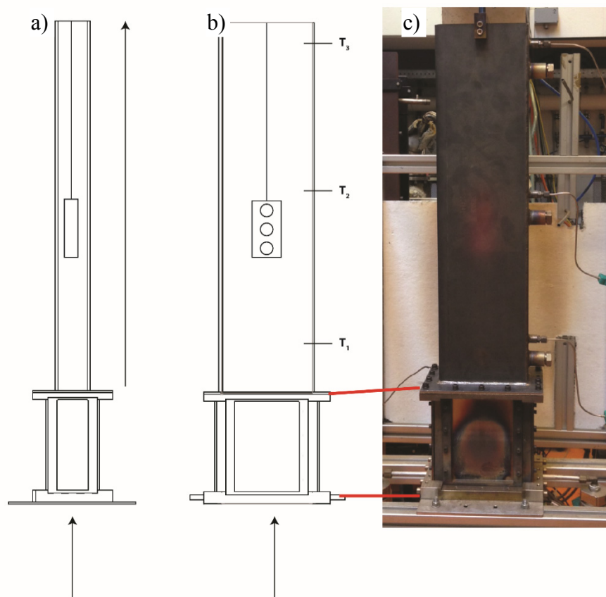
Figure 8.3. Combustion setup: (a) schematic side view with arrows indicating gas flow direction, (b) front view showing the position of the sample holder and thermocouples and (c) actual experimental setup.
