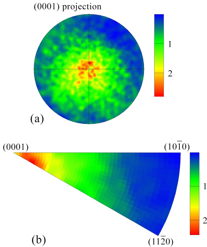
Figure 2.7 Preferred crystallographic orientation of ball milled PLS \text{Cr}_2\text{AlC} to 8 \mu\text{m} grains and subsequently SPS. (a) (0001)-Pole figure and (b) inverse pole figure, both with respect to the sample surface normal (i.e. sintering compaction direction).
