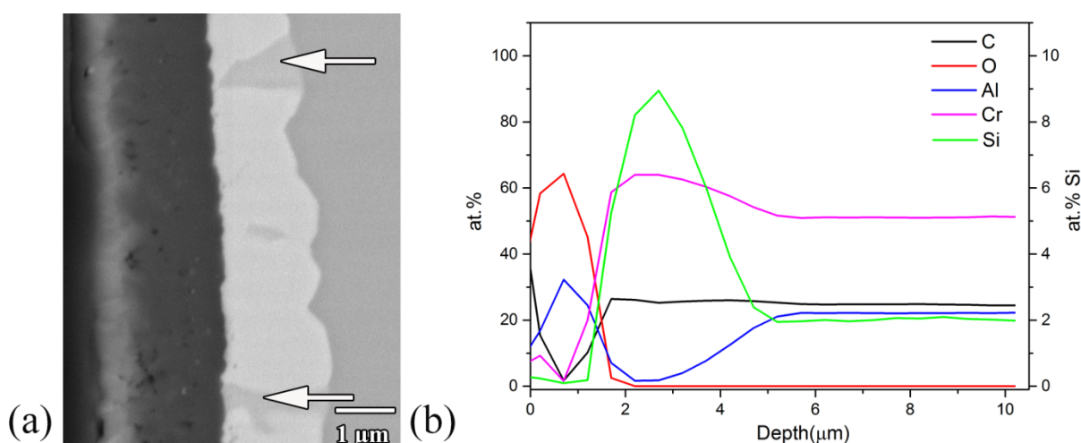
Figure 3.9 (a) BSE image of cross section of Si doped sample \text{Cr}_2\text{Al}_{(0.93)}\text{Si}_{(0.07)}\text{C} after 10 h oxidation in dry synthetic air. The arrows indicate the area where the Si accumulated in the depletion zone; (b) Concentration depth profile recorded with EPMA.
