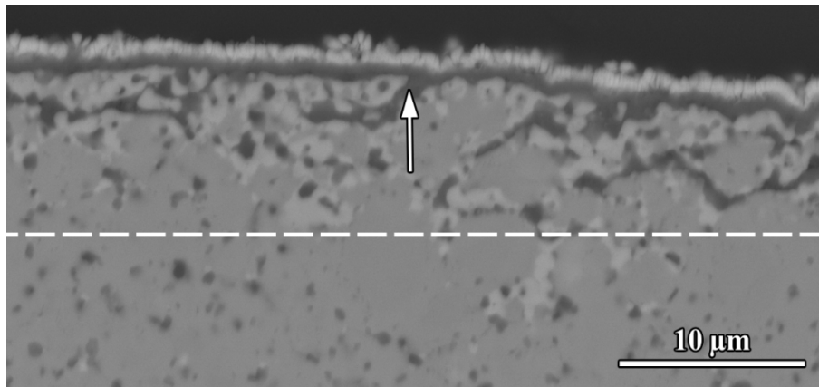
Figure 6.5 SEM image (backscattered electrons) of cross section of \text{Cr}_2\text{AlC} eroded for 60 minutes with 2 g/min spherical glass beads having an average diameter of 95 \mu\text{m} and 110 m/s impact velocity and after oxidation treatment at 1200 ^{\circ}\text{C} in air for 10 minutes. The arrow indicates the healing by \text{Al}_2\text{O}_3 and the dash line marks the healed damage zone. The light phase represents the Al depleted \text{Cr}_2\text{AlC} which is \text{Cr}_7\text{C}_3 . On top of the surface a 0.5 \mu\text{m} copper layer was deposited.
