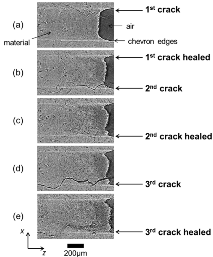
Figure 4.2 Virtual 2D sections through the tomographic datasets showing the sequence of crack growth and healing steps in \text{Ti}_2\text{AlC} at 1500 K in air. Mid-section of the sample: (a) first crack, (b) second crack and healed first crack, (c) healed second crack, (d) third crack and reopening of healed second crack, (e) healed third crack.
