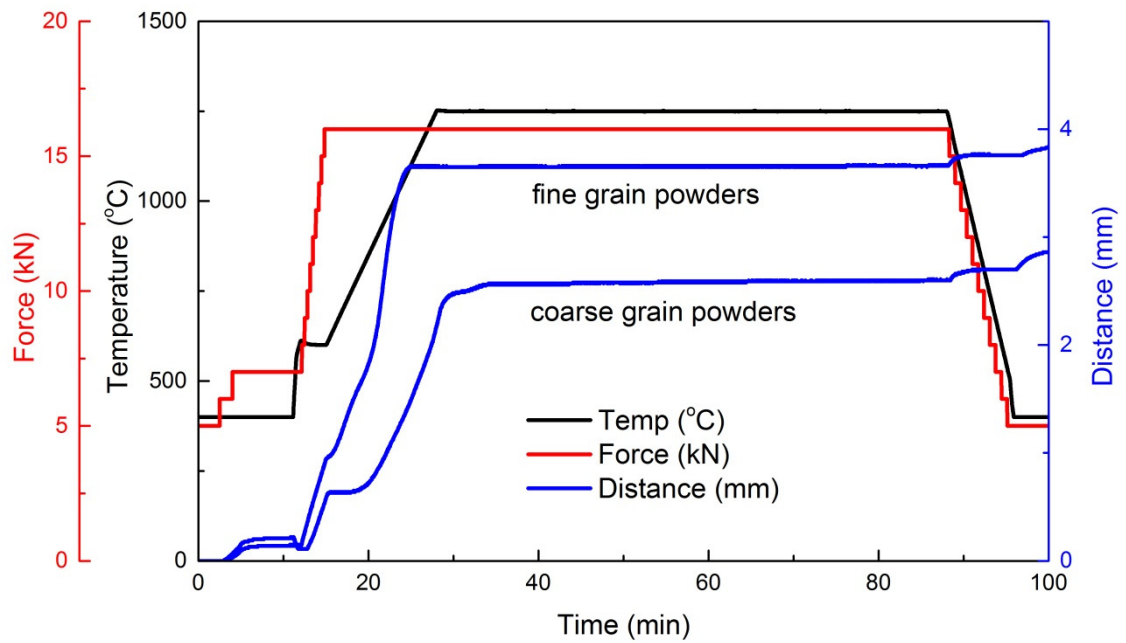
Figure 2.3 Force, temperature and piston travel (distance) during SPS of PLS \text{Cr}_2\text{AlC} powders with coarse and fine grain sizes. The corresponding sintering pressure equals 50 MPa (diameter of the graphite mold is 20 mm).
