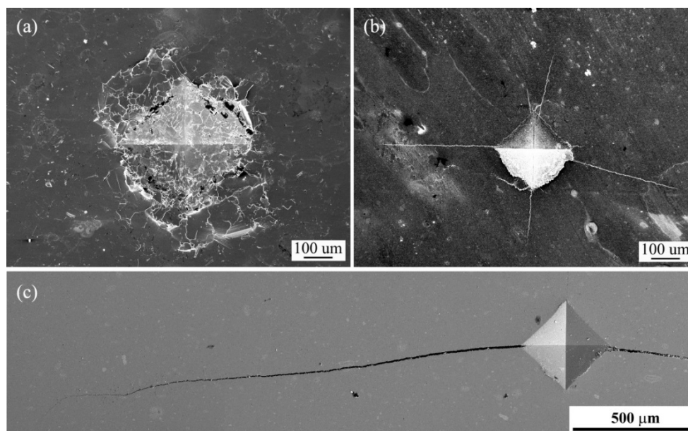
Figure 2.9 Morphologies of Vickers indentations of (a) coarse-grained \text{Cr}_2\text{AlC} bulk ceramic and (b) fine-grained \text{Cr}_2\text{AlC} bulk ceramic surfaces perpendicular and (c) parallel to the sintering compaction direction.
