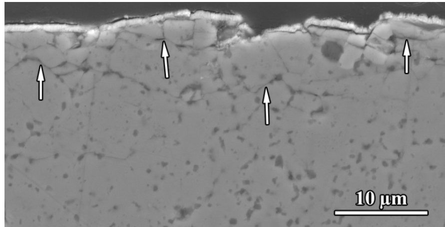
Figure 6.3 SEM image of cross section of eroded sample after 60 minutes with 2 g/min spherical glass beads having an average diameter of 95 \mu\text{m} and 110 m/s impact velocity showing the network of cracks generated. The arrows indicate cracks induced by impacting particles. On top of the surface a 0.5 \mu\text{m} copper layer was deposited.
