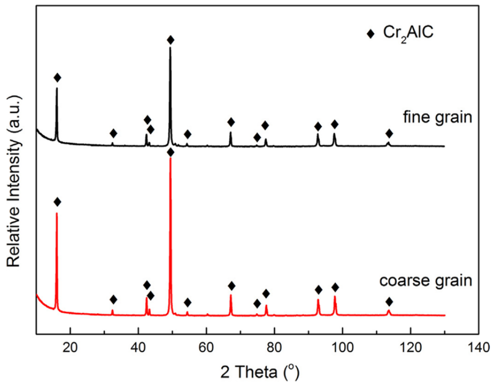
Figure 2.4 X-ray diffractograms of SPS \text{Cr}_2\text{AlC} bulk ceramics with coarse and fine grain size.
