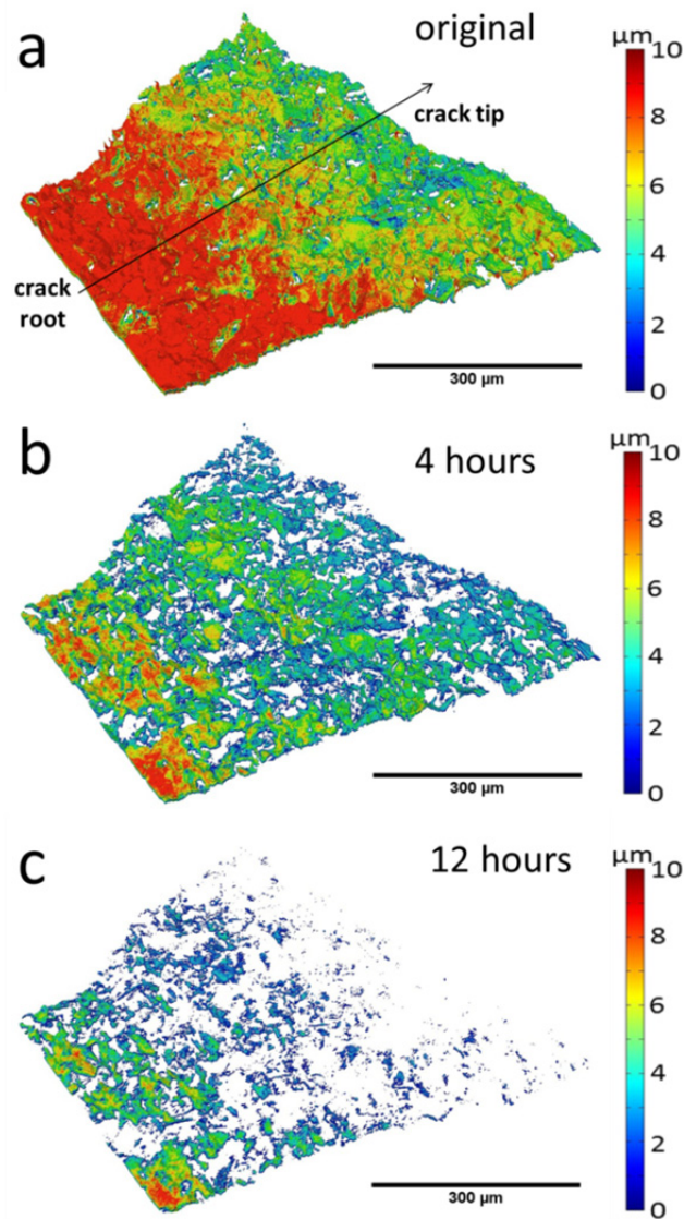
Figure 5.4 3D crack face gap maps (measured in microns) calculated for increasing exposure times: (a) as-cracked; (b) after 4 hours and (c) after 12 hours' healing at 1200 °C in air.
