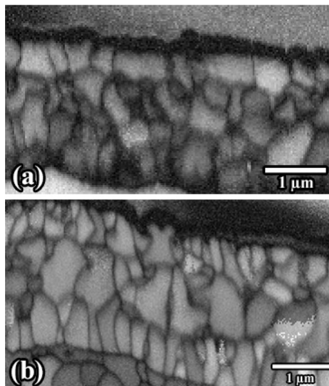
Figure 3.10 Band contrast images of cross section of oxide layer grown on (a) \text{Cr}_2\text{AlC} and (b) \text{Cr}_2\text{Al}_{(0.93)}\text{Si}_{(0.07)}\text{C} surface after oxidation for 10 h in dry synthetic air at 1200 °C.
