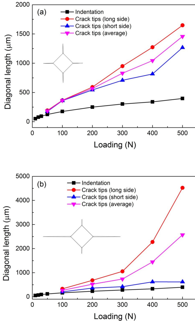
Figure 2.10 Indentation diagonal length and crack tips length of fine-grained Cr_2AlC bulk ceramic as the function of loading in the direction perpendicular (a) and parallel (b) to the sintering compaction direction.
