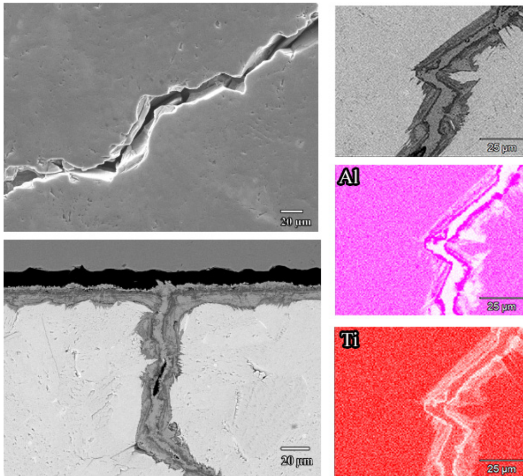
Figure 8.6. (a) Cracks in Ti_2AlC-A after quenching in water from 850\text{ }^\circ C ; (b) cross-section of healed crack after exposure to combustion conditions for 4 hours; (c) close up of healed crack; (d) Al x-ray map; (e) Ti X-ray map.
