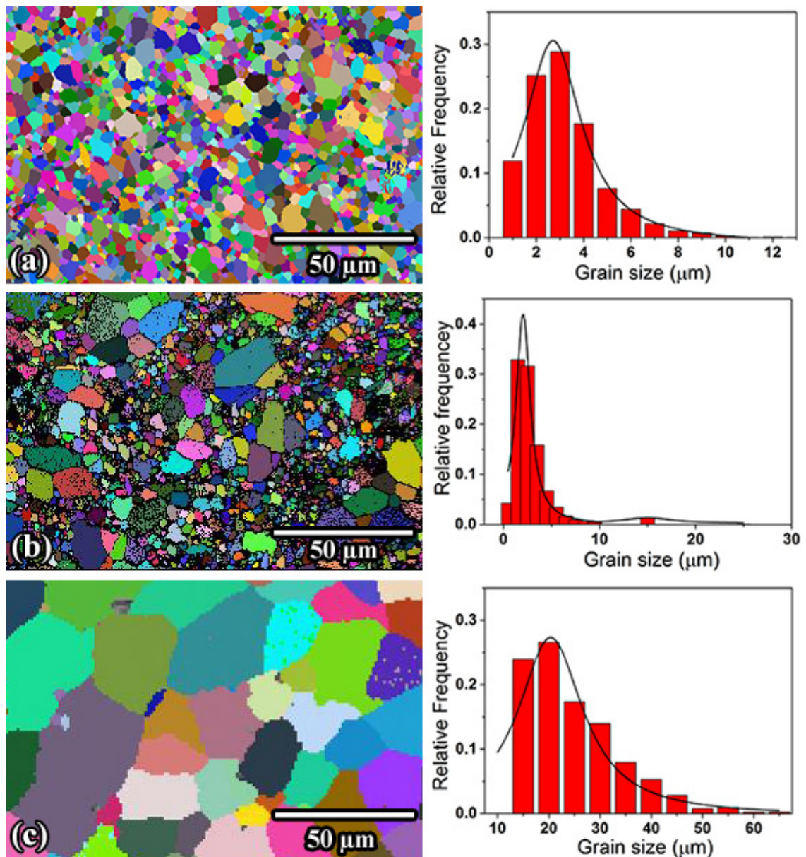
Figure 7.2 Euler maps and grain size distribution graphs of (a) fine-grained, (b) bimodal -grained and (c) coarse-grained \text{Cr}_2\text{AlC} .
