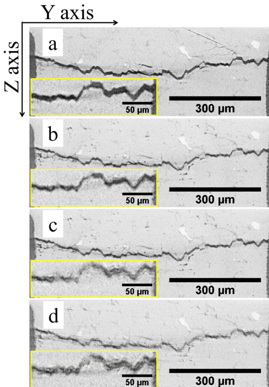
Figure 5.2 2D X-ray tomographic virtual cross-sections through the crack, grown in the X-direction at different stages of healing: (a) as-cracked; (b) after 4 hours; (c) after 8 hours; and (d) after 12 hours exposure to 1200 °C in air. Magnified regions of the crack are shown inset
