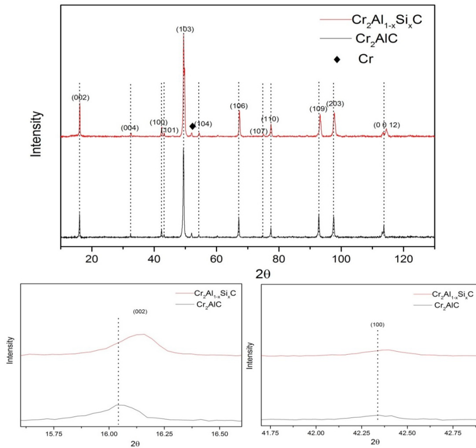
Figure 3.1 XRD patterns of SPS \text{Cr}_2\text{AlC} , and \text{Cr}_2(\text{Al}_{1-x}\text{Si}_x)\text{C} as well as a close look of the (002) and (100) peak shift which corresponds to lattice parameter c and a , respectively.
