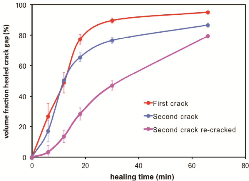
Figure 4.6 Crack healing kinetics in Ti_2AlC at 1500 K in air, presented in terms of volume fraction of the initial crack gap filled with oxide as a function of time. The first and second crack reflect healing in pristine material, while the third crack shows healing of the re-cracked and re-healed second crack (cf. Figure 4.2).
