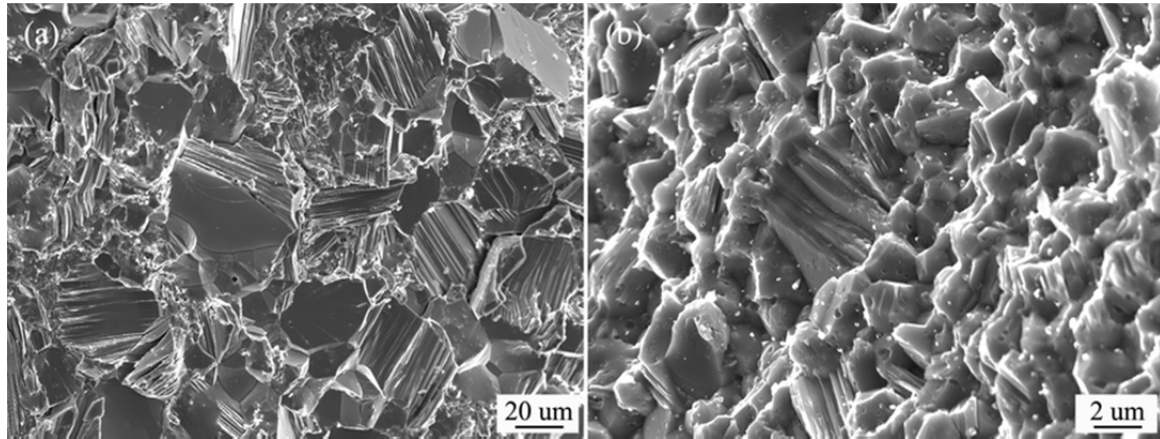
Figure 2.6 SEM images of fracture surfaces of (a) coarse-grained and (b) fine-grained \text{Cr}_2\text{AlC} bulk ceramics.
