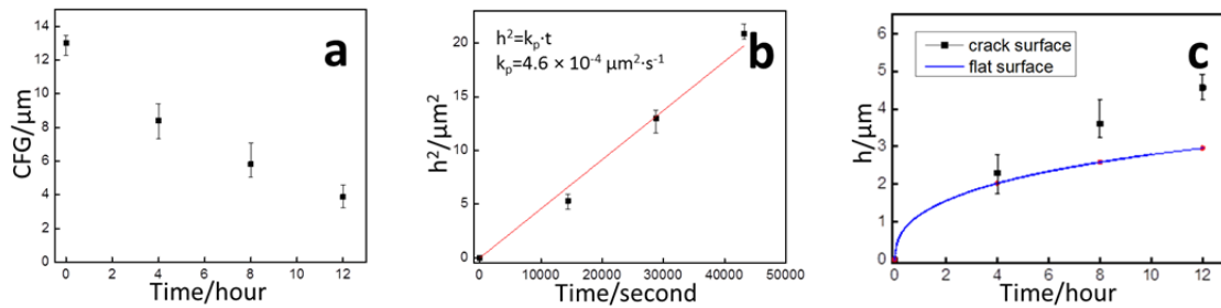
Figure 5.10 (a) Crack face gap at crack root as a function of healing time determined from five 2D virtual X-ray CT slices. (b) Square of the healed crack width ( h ) as a function of healing time. (c) Oxide scale thickness as a function of time on serrated crack surface and flat surface. The TGA experiment was conducted using the same batch of \text{Cr}_2\text{AlC} material under the same oxidation conditions, i.e. at 1200^\circ\text{C} in air.
