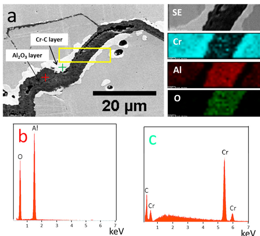
Figure 5.5 (a) Secondary electron cross-sectional SEM image and corresponding elemental maps of crack area after healing at 1200 °C in air for 4h. (b-c) X-ray spectra acquired at the locations indicated by red and green crosses in Figure 5(a) respectively.
