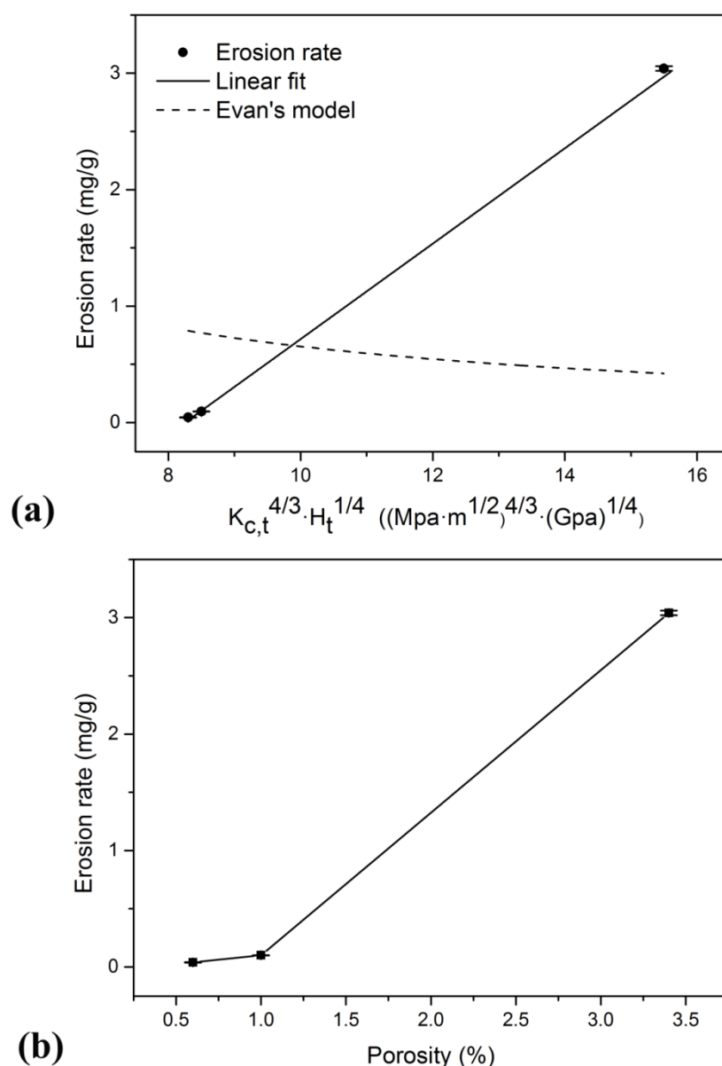
Figure 7.6 Erosion rate as a function of material property factor (product of toughness and hardness, ) (a), and as a function of porosity (b). The material properties dependence according to the Evans' model is indicated by a dashed line in figure a).
