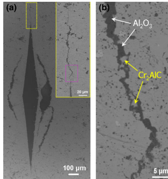
Figure 1.5 Backscattered electron images of polished \text{Cr}_2\text{AlC} after healing at 1100^\circ\text{C} for (a–b) 4 h. (a) low magnification image of the healed zones around indentation on the polished surface. The insert is an enlarged image taken from the marked area in (a). (b) an enlarged image taken from the marked area in the inset in (a). [14]
