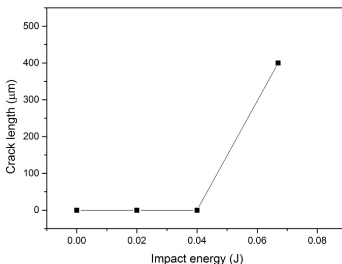
Figure 8.2 Crack length versus impact energy for cracks created in coarse grained \text{Cr}_2\text{AlC} by impact of WC balls.
