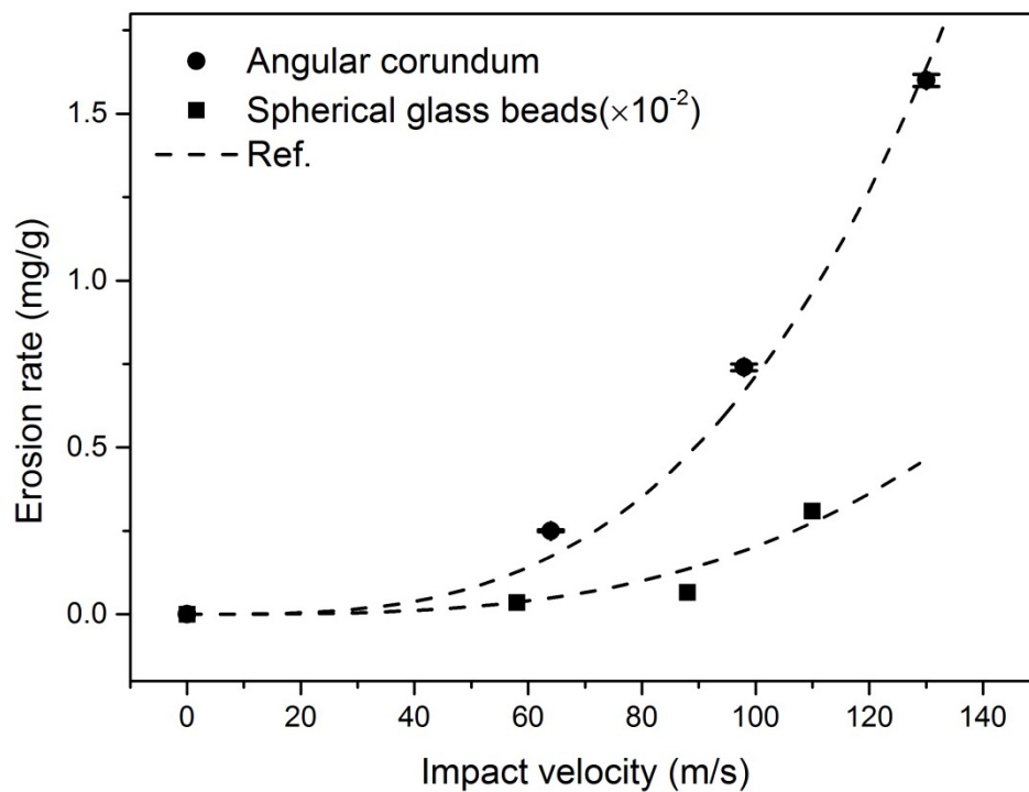
Figure 7.3 Correlation between erosion rate and impact velocity of fine grained \text{Cr}_2\text{AlC} under normal impact with angular corundum with a flux of 2 g/min at a velocity of 130 m/s, 98 m/s and 64 m/s and with micro glass beads under 110 m/s, 88 m/s and 58 m/s with a flux of 5 g/min respectively. The Evans model was fitted to the data points making the exponent the free variable (see text for details).
