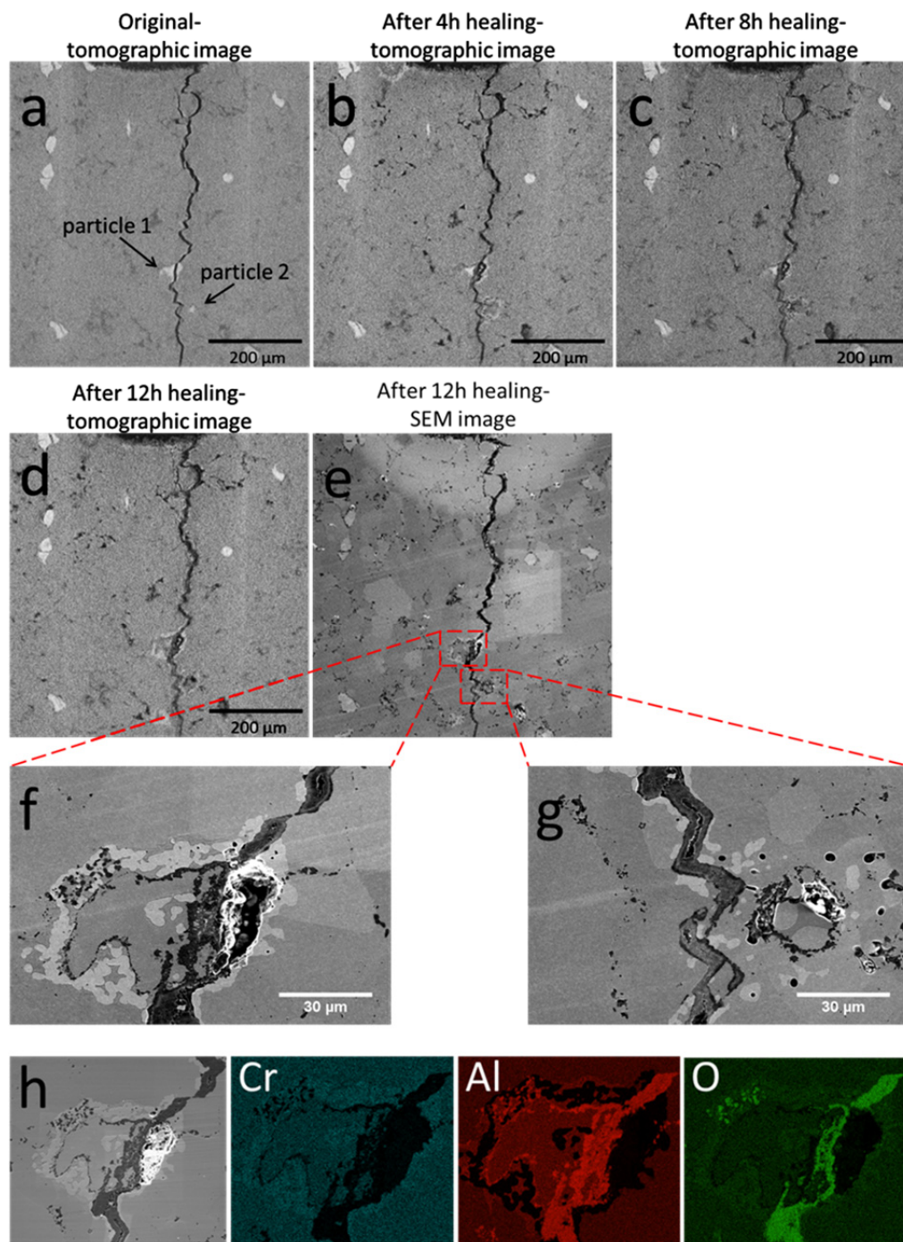
Figure 5.11 (a-d) Time lapse sequence of virtual X-ray tomographic slices of the same region-of-interest as a function of healing time (crack grew from top to bottom) at 1200 °C in air. (e) Secondary electron SEM cross section of the same region-of-interest correlated to (d). (f-g) Higher magnification SEM images of the healed regions indicated by the red rectangles in (e). (h) EDS elemental maps of the region in (f). Particle 2 lies predominantly below the current virtual slice.
