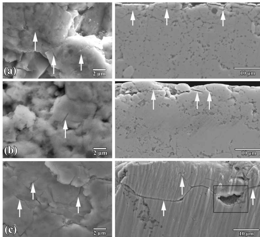
Figure 7.5 SEM images of surfaces (left) and cross section (right) after erosion at 110 m/s with a flux of 2 g/min on (a) fine-grained, (b) bimodal-grained with 100 \mu\text{m} micro glass beads and (c) coarse-grained \text{Cr}_2\text{AlC} with 50 \mu\text{m} micro glass beads. Arrows indicate microcracks generated upon impact, the pores in the coarse grained \text{Cr}_2\text{AlC} are within the black rectangle.
