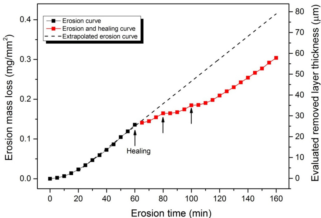
Figure 6.6 The recorded mass loss and evaluated removed layer thickness as a function of erosion time of continuous erosion of virgin \text{Cr}_2\text{AlC} material (black dots). The steady state erosion is extrapolated (dashed line) for comparison. Next, cyclic erosion and healing (red dots) with a cycle of 10 minutes oxidation at 1200^\circ\text{C} in air (indicated with arrows) and of 20 minutes erosion. Then, erosion was continued for another 60 minutes. Erosion by 2 g/min spherical glass beads having an average diameter of 95\ \mu\text{m} and 110 m/s impact velocity.
