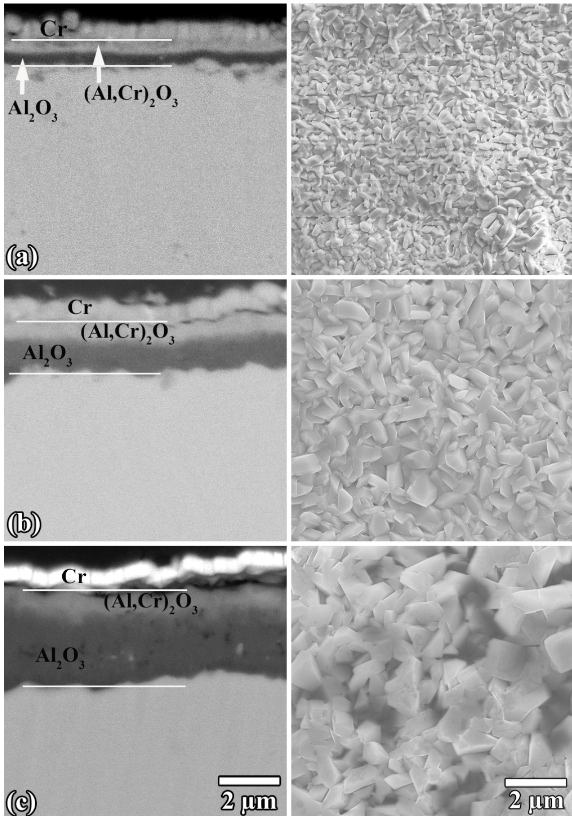
Figure 3.3 The cross section and surface morphology of \text{Cr}_2\text{AlC} after oxidation at (a) 1000, (b) 1100 and (c) 1200 °C in dry synthetic air for 10 h with the same magnification. A 0.5 \mu\text{m} thick Cr was deposited at the oxidized sample surface.
