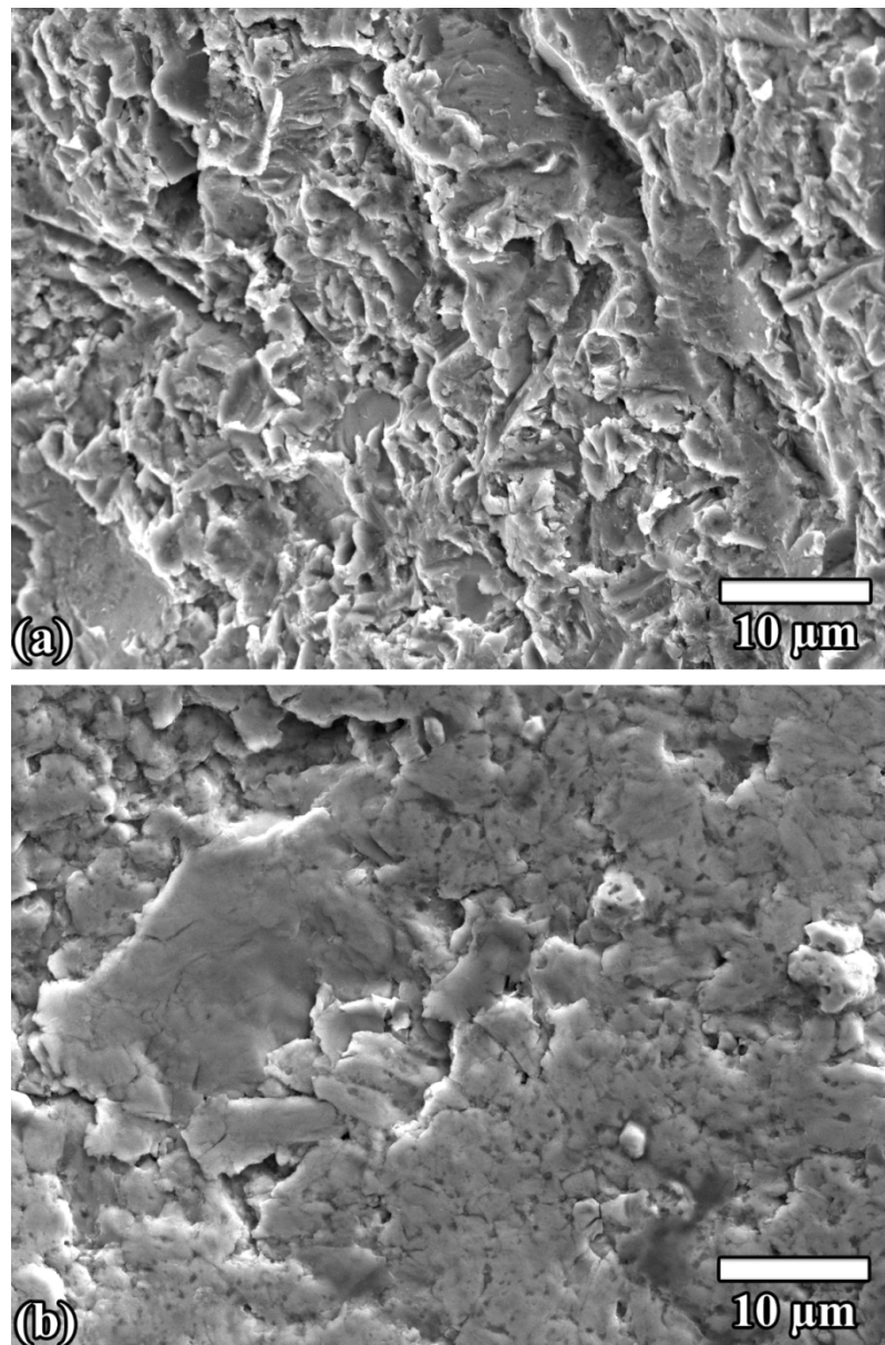
Figure 7.4 Eroded surface morphology of fine-grained \text{Cr}_2\text{AlC} after erosion for 60 min. with (a) 2 g/min angular corundum at 130 m/s, and (b) 5 g/min micro glass beads at 110 m/s.
