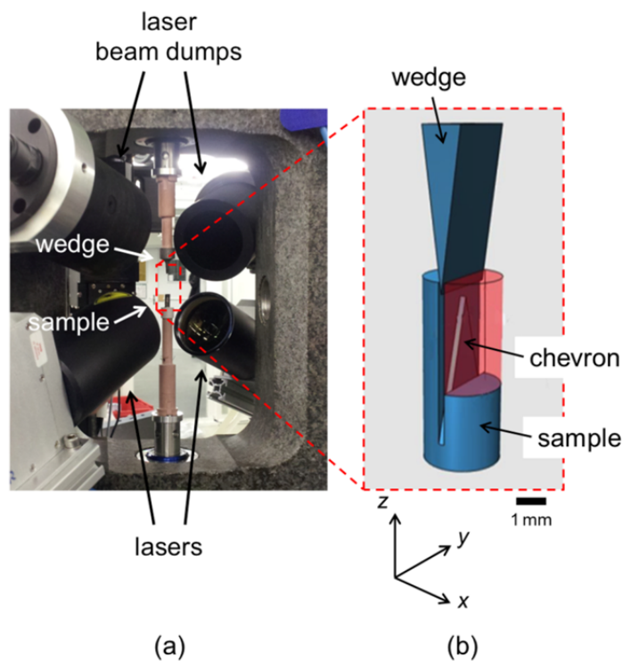
Figure 4.1 Thermomechanical testing rig for in situ 4D X-ray tomographic microscopy. (a) Image of the mechanical testing rig incorporating the laser-based heating system mounted at the TOMCAT beamline; the sample stage and wedge setup are also visible. (b) Sample and wedge configuration; the arrow indicates the chevron where the cracks are generated and healed.
