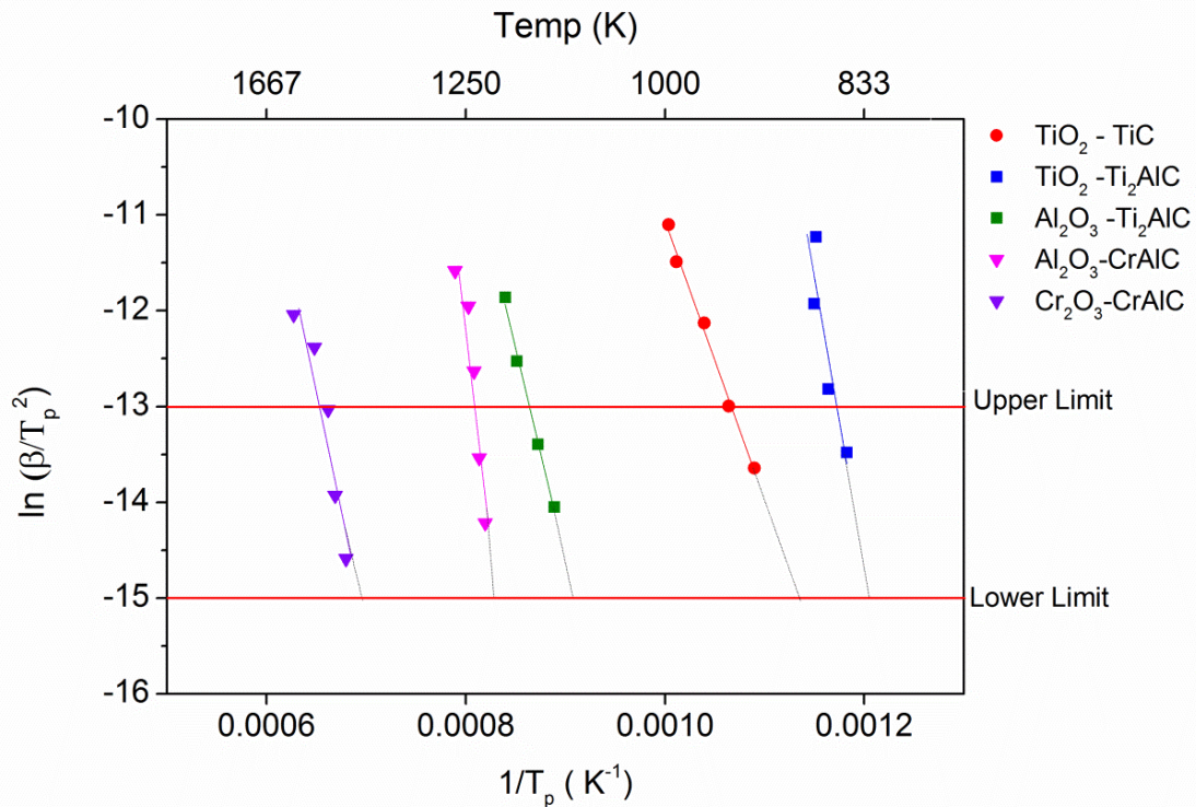
Figure 8.4. Evaluating the activation energy for the different reactions occurring during oxidation of all healing materials considered (Plot of reactivity versus peak temperature).
