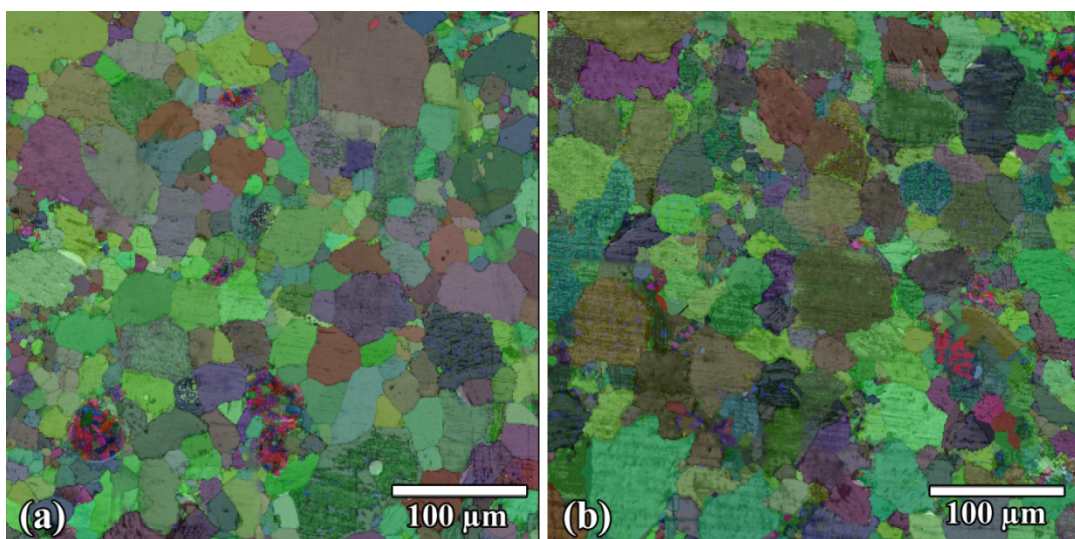
Figure 3.2 Euler maps of bulk (a) \text{Cr}_2\text{AlC} and (b) \text{Cr}_2\text{Al}_{(0.93)}\text{Si}_{(0.07)}\text{C} .
