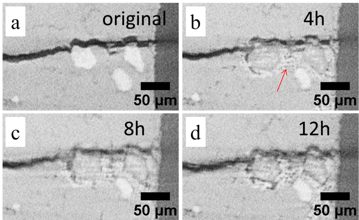
Figure 5.3 2D X-ray tomographic cross sections with surface breaking Cr particles at different healing stages: (a) original; (b) after 4 hours healing at 1200\ ^\circ\text{C} in air; (c) after 8 hours healing at 1200\ ^\circ\text{C} in air; (d) after 12 hours healing at 1200\ ^\circ\text{C} in air.
