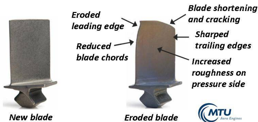
Figure 1.1 Turbine blade before (left) and after (right) operation with named damages. After [5]
