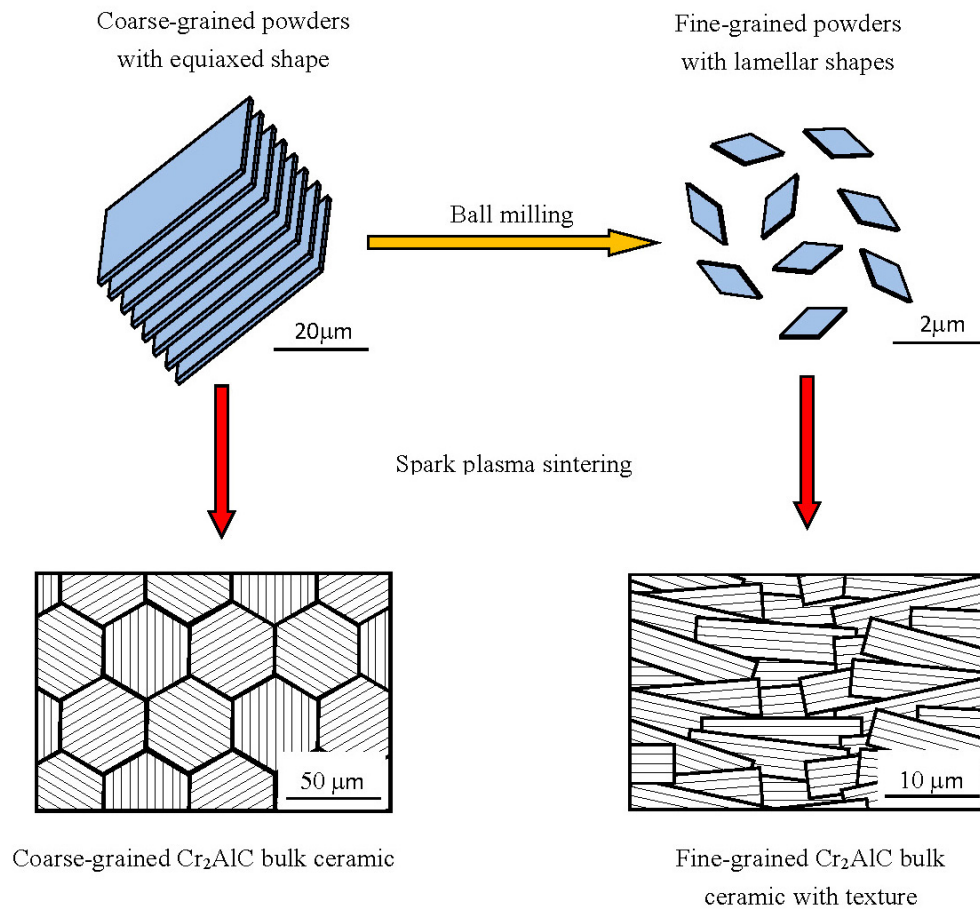
Figure 2.8 Schematic representation of the microstructures evolution, consequently upon PLS of \text{Cr}_2\text{AlC} , ball-milling and SPS.
