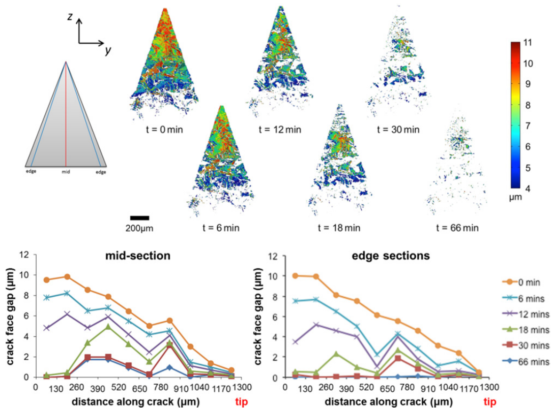
Figure 4.3 Planar views of the 3D datasets segmented to show the first crack in Ti_2AlC both initially and at different stages of healing at 1500 K in air. This first crack (cf. Figure 4.2) has a length of 1.2 mm. The superimposed colour map represents the crack face gap (CFG). The direction of crack growth is from top (mouth) to bottom (crack-tip) in the images. The graphs show the remaining opening of the crack having a length of 1.2 mm as a function of healing time for virtual sections in the middle and towards the edges of the crack (averaged over both edge trajectories).
