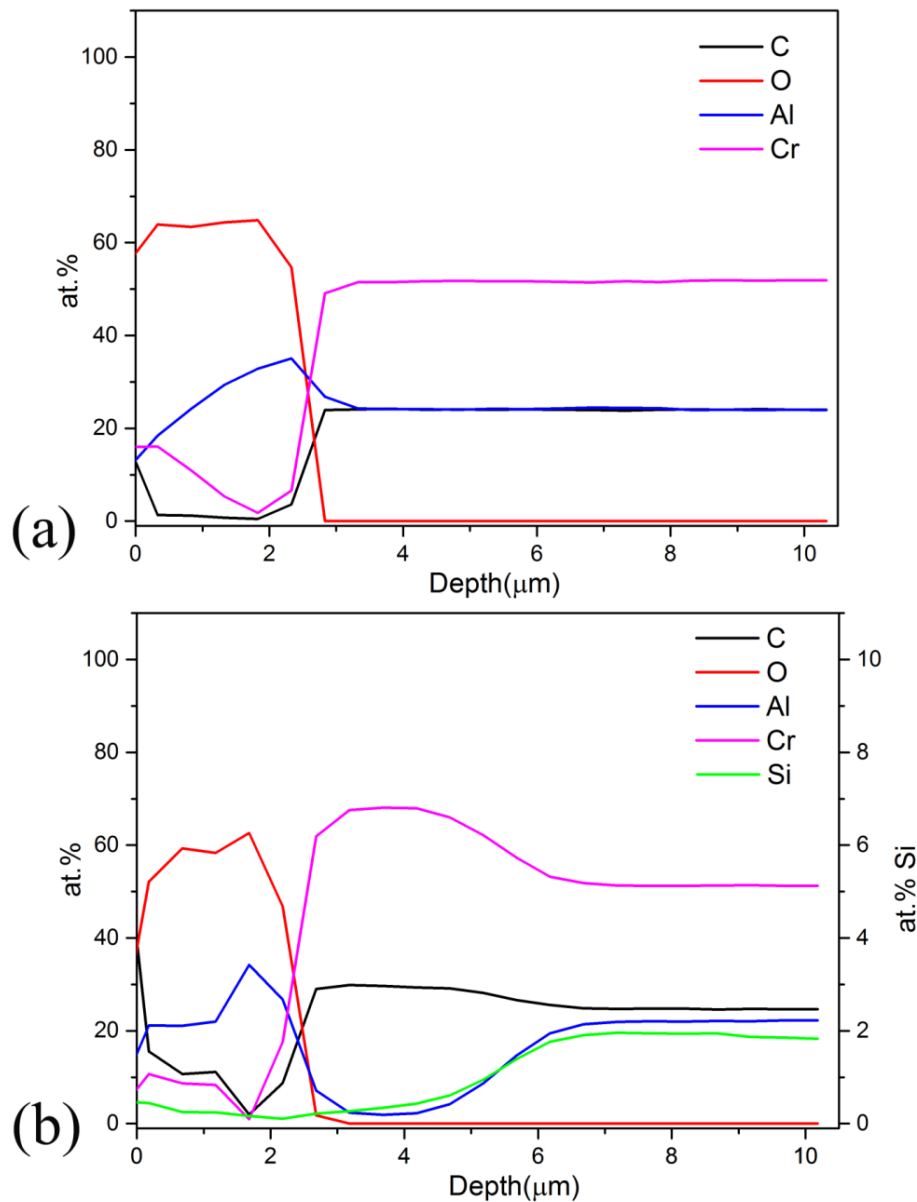
Figure 3.7 Concentration depth profiles after oxidation at 1200 °C for 10 h in dry synthetic air of (a) \text{Cr}_2\text{AlC} and (b) \text{Cr}_2\text{Al}_{(0.93)}\text{Si}_{(0.07)}\text{C} from the surface to the matrix (left to right).
