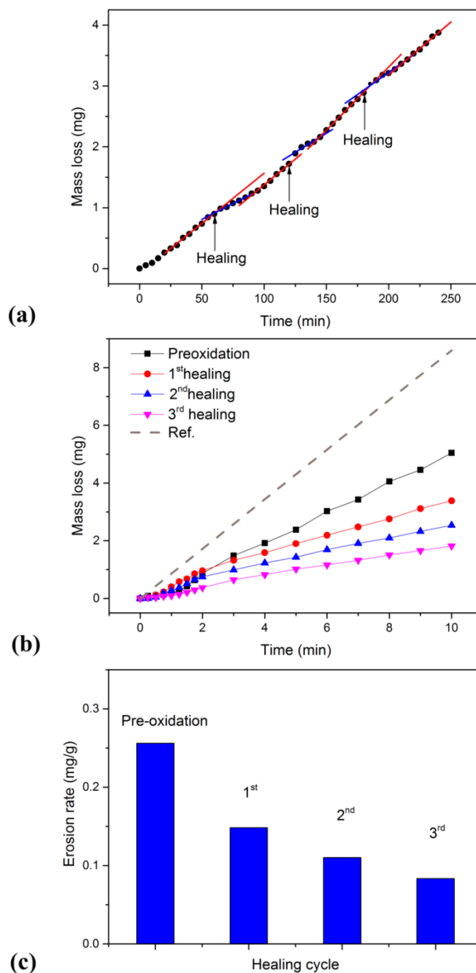
Figure 7.7 Mass loss of (a) fine grained and (b) coarse-grained Cr_2AlC as a function of erosion time due to impact of 100\ \mu m micro glass beads at 110\ m/s and 2\ g/min . After each erosion cycle a healing treatment was executed at 1200\ ^\circ C in air for 10\ min . The coarse-grained Cr_2AlC was oxidized at 1200\ ^\circ C in air for 10\ min . prior to the cyclic erosion test. The dash line shows the erosion rate of the as produced coarse-grained Cr_2AlC . (c) Change of erosion rate of the coarse-gained Cr_2AlC after pre-oxidation and each healing treatment.
