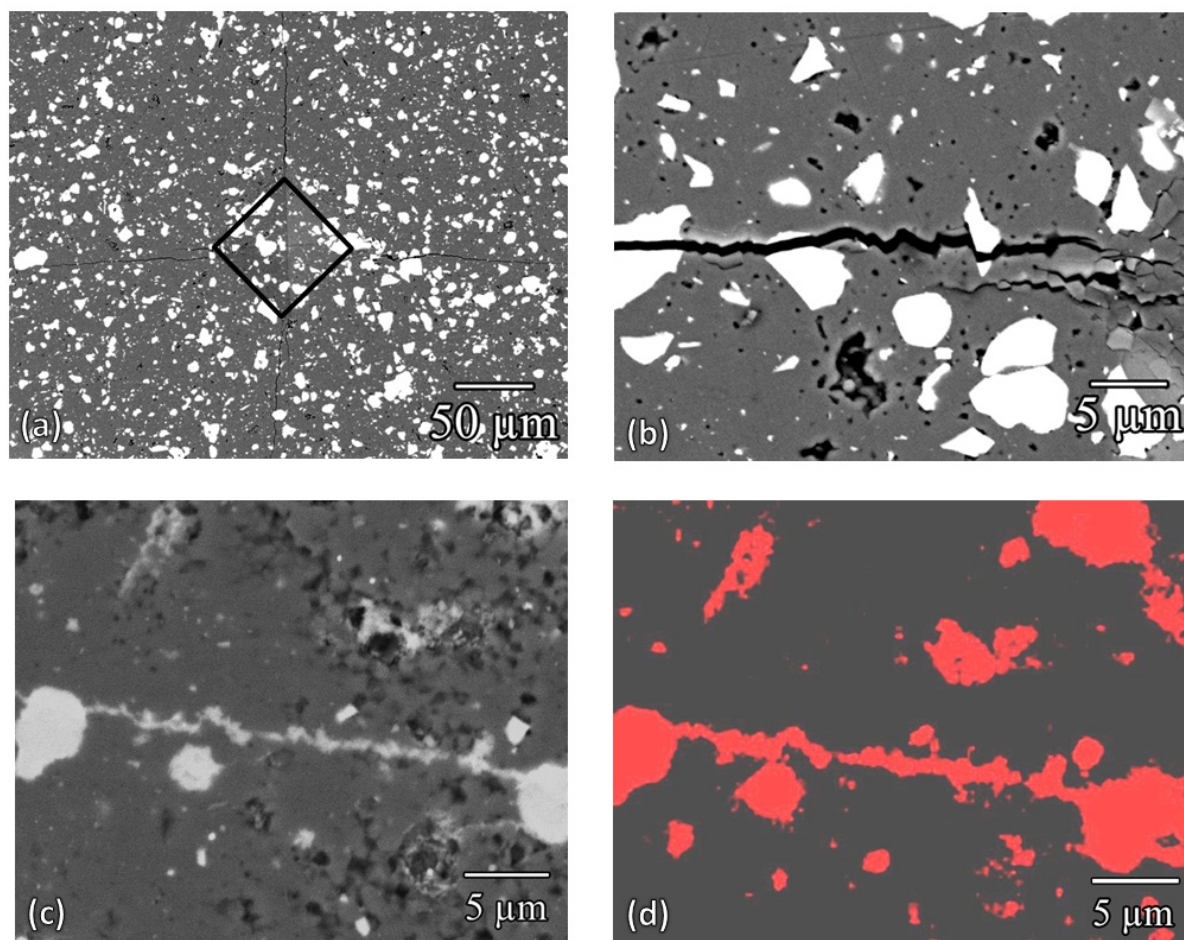
Figure 8.5. SEM micrographs of Al_2O_3/TiC composite. (a) Cracks created by Vickers indentation; (b) close-up showing crack-particle interaction, (c) healed crack after exposure to combustion environment for 4 hours, (d) Ti X-ray mapping showing the filling of the healed crack.
