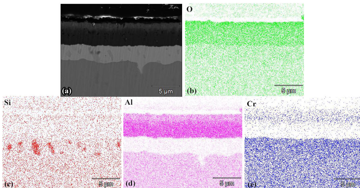
Figure 3.8 (a) BSE image of a cross section of \text{Cr}_2\text{Al}_{(0.93)}\text{Si}_{(0.07)}\text{C} after oxidation in dry synthetic air for 10 h at 1200 °C, (b) O X-ray map, (c) Si X-ray map, (d) Al X-ray map, (e) Cr X-ray map.
