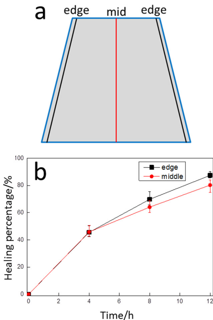
Figure 5.7 (a) Lines along which the percentage healing was quantified. (b) Percentage of crack healing as a function of healing time calculated at middle and edge of the crack, respectively.
