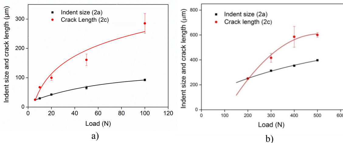
Figure 8.1 Vickers Indent size and crack length versus applied load of (a) \text{Al}_2\text{O}_3 with 20 vol. % TiC composite and (b) fine grained \text{Cr}_2\text{AlC} .
