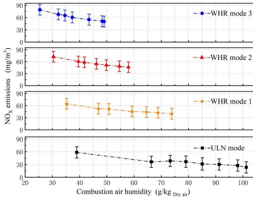
Figure 12. Effect of air humidity on \text{NO}_x emissions.
