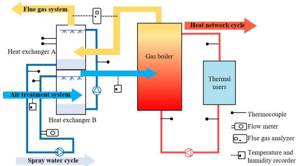
Figure 2. Flow chart of ULN mode of FGLNHR-CAH system.
