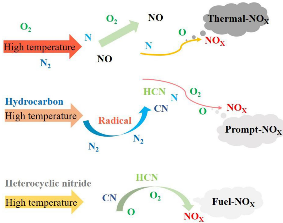
Figure 13. Formation mechanism of \text{NO}_x in gas boiler.
