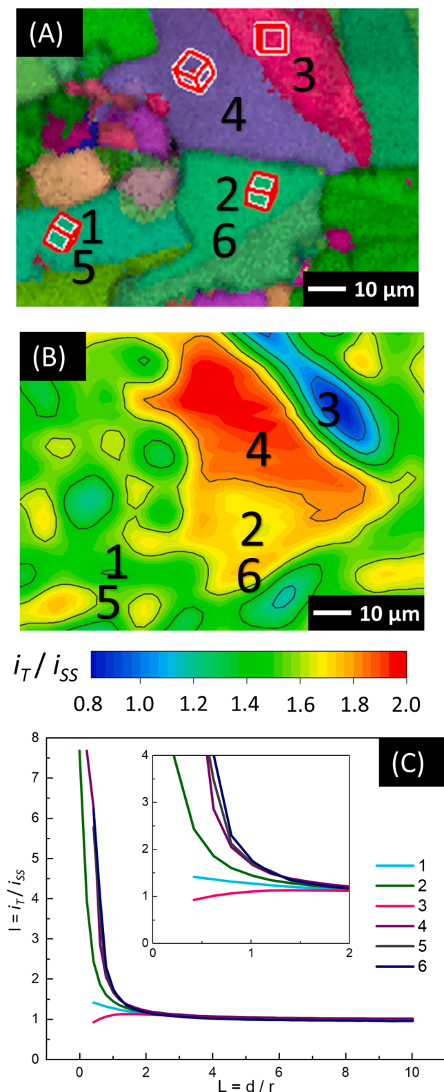
Fig. 6. (A) EBSD orientation map and (B) SECM map ( 100 \times 80 \mu\text{m}^2 ) of the polished growth surface (same area) obtained with a 10 \mu\text{m} diameter Pt tip in 1 mM FcMeOH +/0 (in 0.1 M KNO 3 ), with a tip potential of +0.5 V (vs. Ag/AgCl) and the BDD substrate kept under OCP. (C) Experimental probe approach curves recorded at the six different spots, as indicated by the numbers in (A) and (B).
