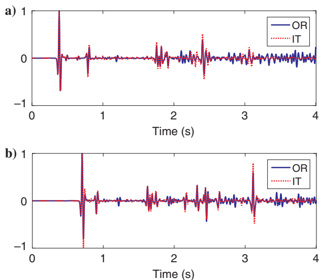
Figure 9. (a) A comparison of zero-offset traces from the original (OR) and retrieved data sets (IT) and (b) a comparison of the non-zero-offset (1000 m) traces.
