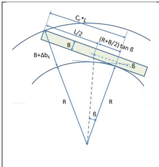
Figure 1 Definition sketch for the extra path width ( \Delta b ) in a bend.
