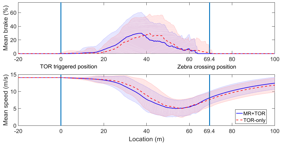
Fig. 7. Means and standard deviations across events of the brake position and driving speed in the take-over scenarios in the MR + TOR and TOR-only conditions as a function of travelled distance. The vertical lines mark the start of the TOR (0 m) and the position of the zebra crossing (69.4 m). Note that these are averages, which means that these graphs cannot be used to make inferences about the behaviour of individual participants. For example, the minimum averaged speed in this graph is about 5 m/s, while the majority of the participants came to a full stop.
