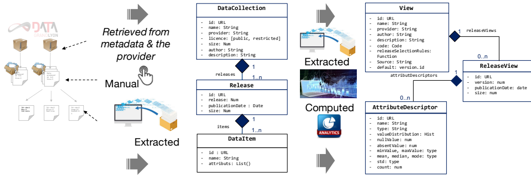
Figure 1: CURARE Model
