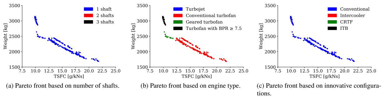
Figure 14 Pareto front of TSFC and weight for the realistic engine architecting problem. The color indications for each graph are indicated in Figures 11 to 13.
