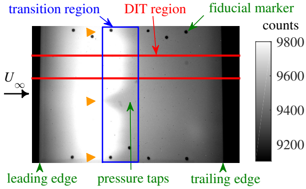
Figure 3: Infrared image for a static case, \alpha = 1.5^\circ .
