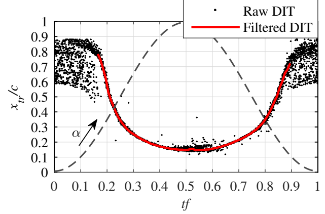
Figure 11: DIT result, \alpha = 4^\circ \pm 7^\circ , k = 0.075 .
