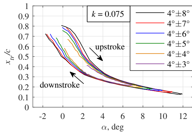
Figure 21: DIT transition results, variation of the pitch amplitude \hat{\alpha} for \bar{\alpha} = 4^\circ and k = 0.075 .
