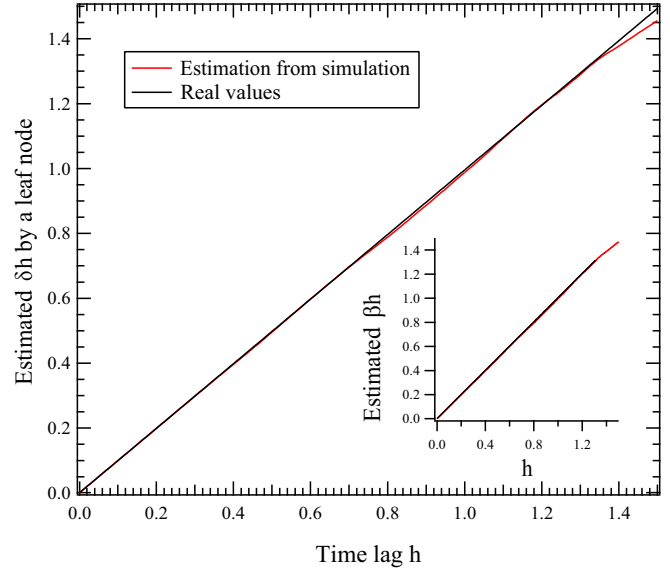
FIG. 8. The estimation of the infection rate \beta and the curing rate \delta using (23) and (22) for the star graph corresponding to Fig. 3. The curves are -(1 - v_{j\infty}) \ln[R_{j\infty}(h)] and -\frac{v_{j\infty} \ln[R_{j\infty}(h)]}{\sum_{i=1}^N a_{ji} v_{i\infty}} of a leaf node versus h . Both the estimated \beta and \delta are 1.00, while the real values of rates are both 1.
