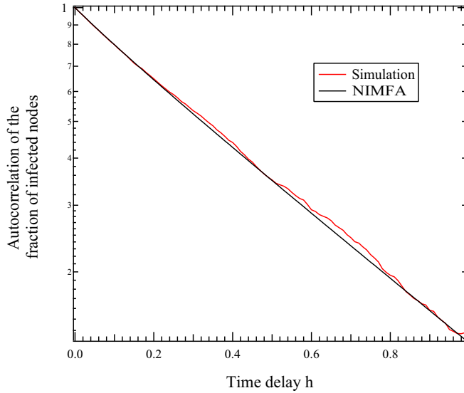
FIG. 7. The autocorrelation of the fraction of infected nodes R_I(0.5, 0.5 + h) and the corresponding NIMFA approximation R_{I^{(1)}}(0.5, 0.5 + h) of the SIS process on the star graph.
