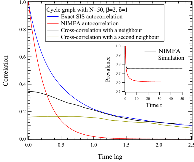
FIG. 4. The correlation of the infection state of a node and the prevalence in a cycle graph with N = 50 . Initially all nodes are infected to prevent the inaccuracy caused by early die-out [24]. The NIMFA autocorrelation is much smaller than the exact one, and the cross correlations between neighbors and second-hop neighbors are very large.
