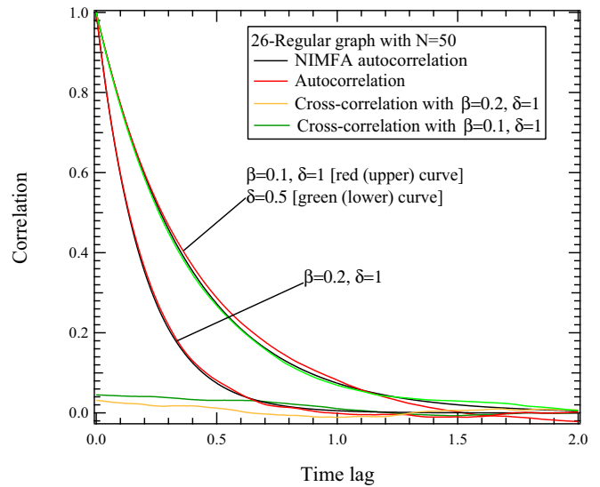
FIG. 2. The autocorrelation of the infection state of a 26-regular graph with N = 50 . The results are similar to those of the ER graph. The autocorrelation is invariant to \delta .
