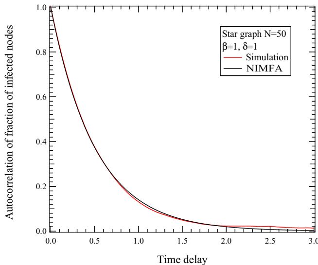
FIG. 5. The autocorrelation of the fraction of infected nodes I(t) in the metastable state.
