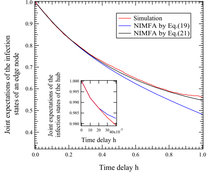
FIG. 6. The joint expectation of the infection state E[X_j(0)X_j(h)] and the corresponding NIMFA approximation E[V_j(0)V_j(h)] of the SIS process on the star graph.
