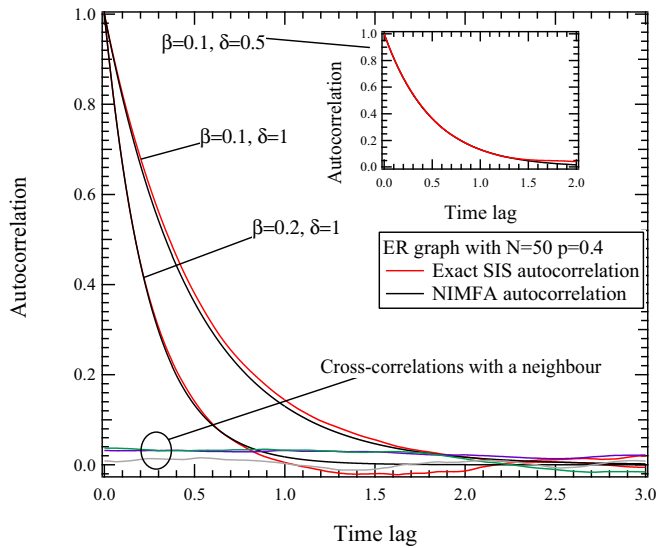
FIG. 1. A randomly selected node is evaluated in an Erdős-Rényi (ER) network with the link connecting probability 0.4 and N = 50 . The autocorrelation is approximately constant for different value of \delta . The cross correlation between the node with one of its neighbors is also plotted, which is almost zero.
