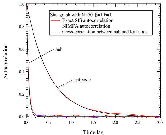
FIG. 3. The autocorrelation of the infection state of the hub and a leaf node in a star graph with N = 50 . The NIMFA autocorrelation shows a very good approximation and the cross correlation between hub and leaf nodes is approximately 0.
