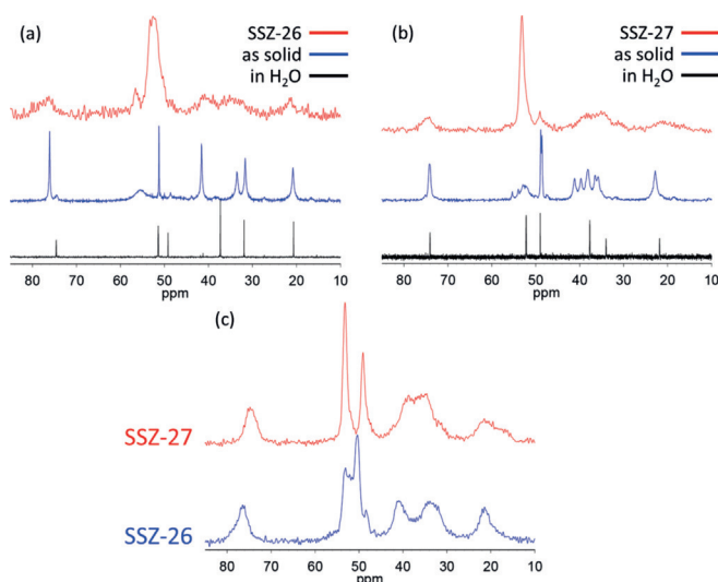
Figure 8. ^{13}\text{C} MAS NMR spectra for a) SSZ-26 (red), isomer I in the solid state (blue) and in water (black), b) SSZ-27 (red), isomer III in the solid state (blue) and in water (black). c) ^{13}\text{C} CPMAS-NMR (0.5 ms cross-polarization contact time) spectra for SSZ-26 and SSZ-27.
