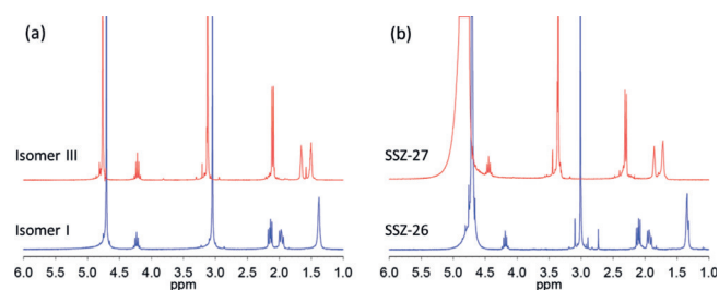
Figure 9. Liquid-phase ^1\text{H} NMR spectra for a) pure isomers I and III, and b) organic compounds extracted after dissolution of SSZ-26 and SSZ-27.
