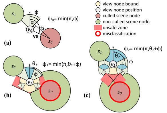
Figure 5: Culling. For a single view (a), we can cull scene nodes outside the view frustum. For multiple views (b), we test by virtually enlarging the scene node bound (large green area behind misclassification). Hereby, we avoid incorrect culling, as for s_0 . We use the same process for nodes with an angular extent 2(\theta_j + \phi) > \pi (c).
