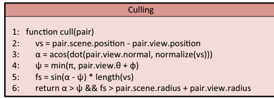
Figure 4: Pseudocode for culling with spherical bounding volumes.
