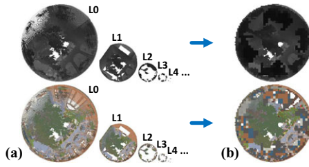
Figure 9: Multi-level point-only renderings at a 256^2 resolution for a single view (a) using mipmap-based hole filling (b).
