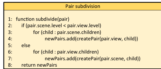
Figure 8: Pseudocode for pair subdivision for octree structures.
