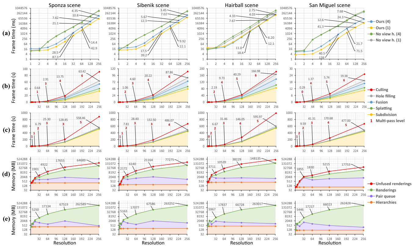
Figure 12: View render timings for four scenes against the rendering resolution (a). We compare our method to not using a view hierarchy (ManyLoDs [HREB11]). Again, we initialized the view set as 1- and 4-bounce VPLs. Data labels denote the average number of single views that share a scene node rendering in (a). We break down the results for individual components of our method (b) and ManyLoDs (c), additionally showing the multi-pass levels as data labels, and show our GPU memory consumption (d) and that for ManyLoDs (e).
