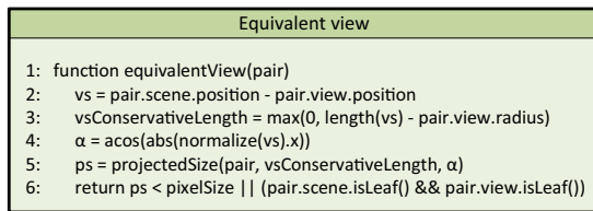
Figure 6: Pseudocode for view equivalence computation for dual paraboloid mapping and spherical bounding volumes.
