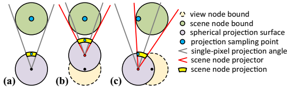
Figure 7: Discrepancies of scene-node projections for vertical (b) and horizontal (c) displacement of a child view against the projection for the centre of the view node (a).
