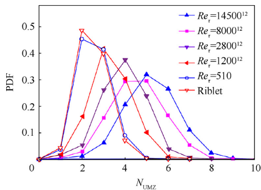
(a) PDF of number of UMZ
