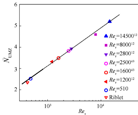
(b) Change of average number of UMZ with Re_\tau
