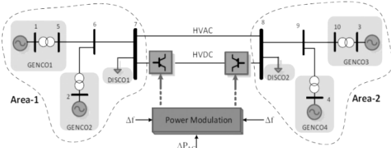
Fig. 2. A schematic diagram of a two-area AGC model with a parallel AC/HVDC link
