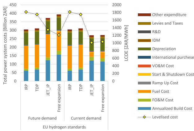
Fig. 7. Total cost and levelized costs of electricity (LCOE) in the 90 gCO 2 /kWh emission constraint enforced scenario. Note that due to high levels of unserved energy, the policy scenarios in this context are considered unfeasible.
