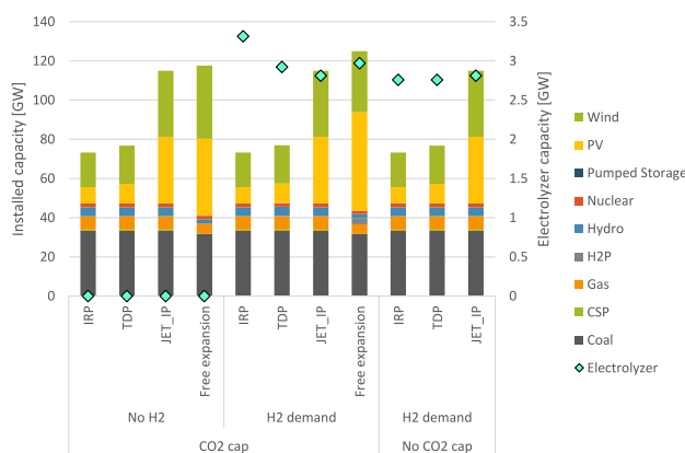
Fig. 3. – Total installed capacities in South Africa 2030.
