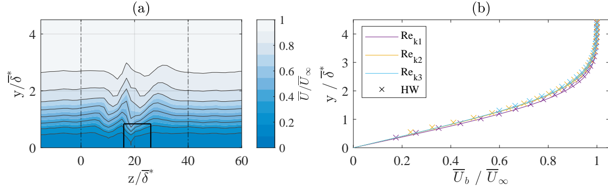
Fig. 1 (a) Time-averaged HWA velocity contours for Re_{k_2} at x/c=0.2 . Velocity isolines every 10% of \bar{U}_\infty (gray lines); sketch of the element location (black rectangle); limits of the perturbed flow region (vertical - lines). (b) Comparison of HWA ( \times ) and numerical (-) boundary layer velocity profile at x/c=0.2 .
