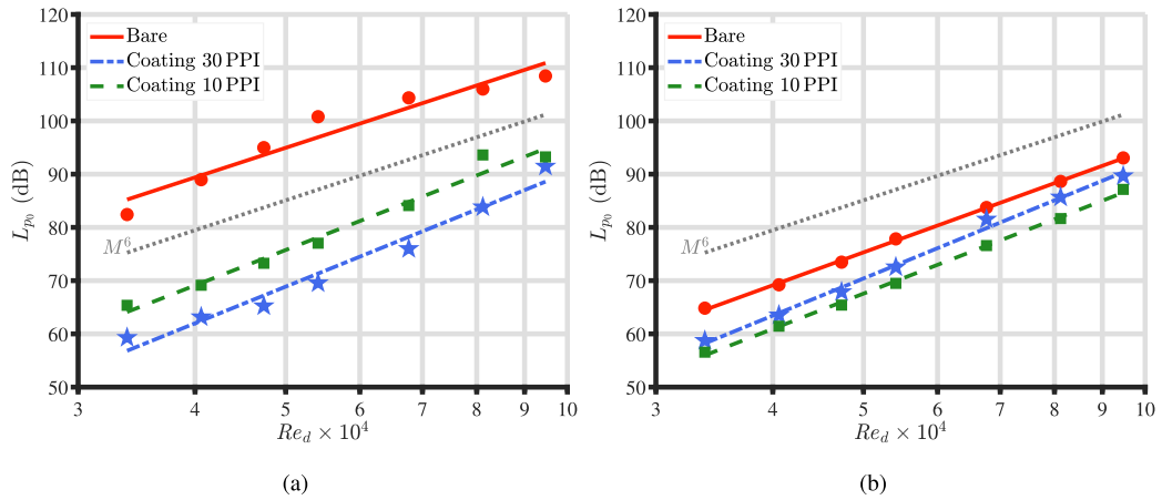
Fig. 8. Overall sound pressure levels ( p_{\text{ref}} = 20 \mu\text{Pa} ) of the (a) tonal and (b) broadband part of the frequency spectrum at different free-stream Reynolds numbers for the three configurations measured by the central microphone of the array. The slope associated with the sixth power of the Mach number, as well as the interpolation of the experimental points using a linear regression model, are also indicated in the plot.
