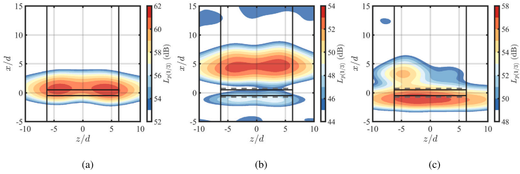
Fig. 12. Source-distribution maps for (a) the baseline and the cylinders coated with the (b) 30 PPI and (c) 10 PPI metal foams at f_{1/3} = 5 kHz and Re_d = 6.8 \times 10^4 ( St = 2 ) computed with p_{ref} = 20 \mu Pa.
