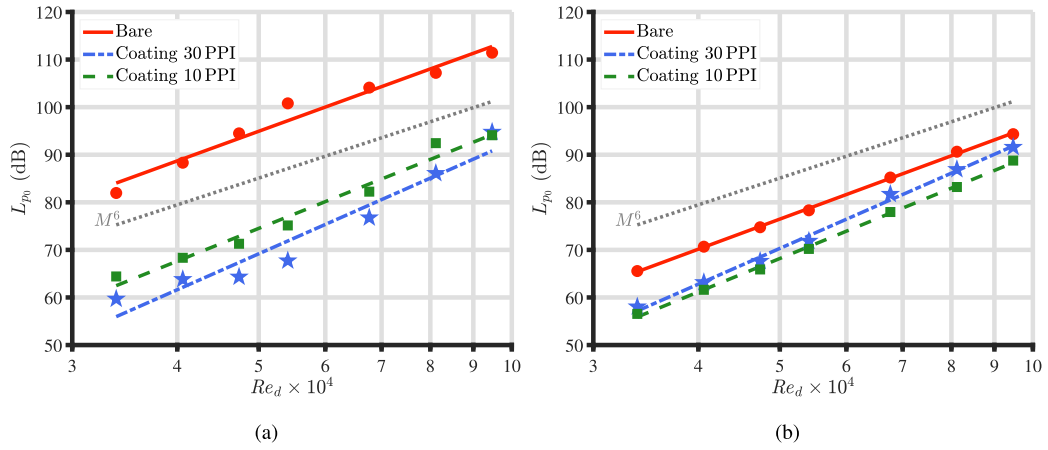
Fig. 9. Overall sound pressure levels ( p_{\text{ref}} = 20 \mu\text{Pa} ) of the (a) tonal and (b) broadband part of the frequency spectrum at different free-stream Reynolds numbers for the three configurations measured by the most downstream microphone of the array. The slope associated with the sixth power of the Mach number, as well as the interpolation of the experimental points using a linear regression model, are also indicated in the plot.
