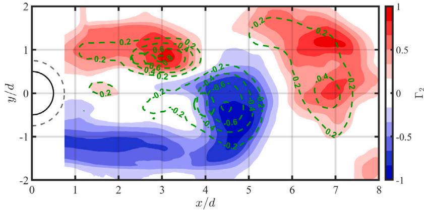
Fig. 16. \Gamma_2 function field for the cylinder coated with the 30 PPI metal foam at Re_d = 6.8 \times 10^4 corresponding to the instantaneous magnitude-velocity field in Fig. 5. The green dashed lines denote the values of the \Gamma_1 function.
