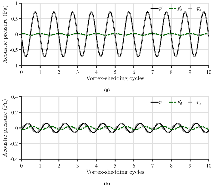
Fig. 23. Time series of the total, direct, and scattered acoustic pressure radiated at the vortex-shedding frequency by (a) the baseline and (b) the cylinder coated with the 30 PPI metal foam at Re_d = 6.8 \times 10^4 at the location of the central microphone of the array.
