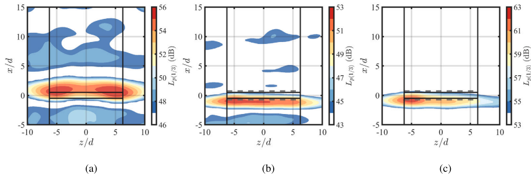
Fig. 13. Source-distribution maps for (a) the baseline and the cylinders coated with the (b) 30 PPI and (c) 10 PPI metal foams at f_{1/3} = 8 kHz and Re_d = 6.8 \times 10^4 ( St = 3.2 ) computed with p_{ref} = 20 \mu Pa.
