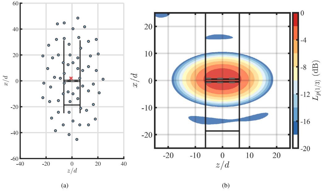
Fig. 3. (a) Relative position of the microphone array and the test section. The solid lines indicate side plates, nozzle exit, and cylinder leading edge and trailing edge. The central microphone of the array is denoted by the red x symbol. (b) Point-spread function at f_{1/3} = 1.25 kHz for a simulated source emitting white noise at the origin of the coordinate system. The flow goes from the bottom to the top of the maps.
