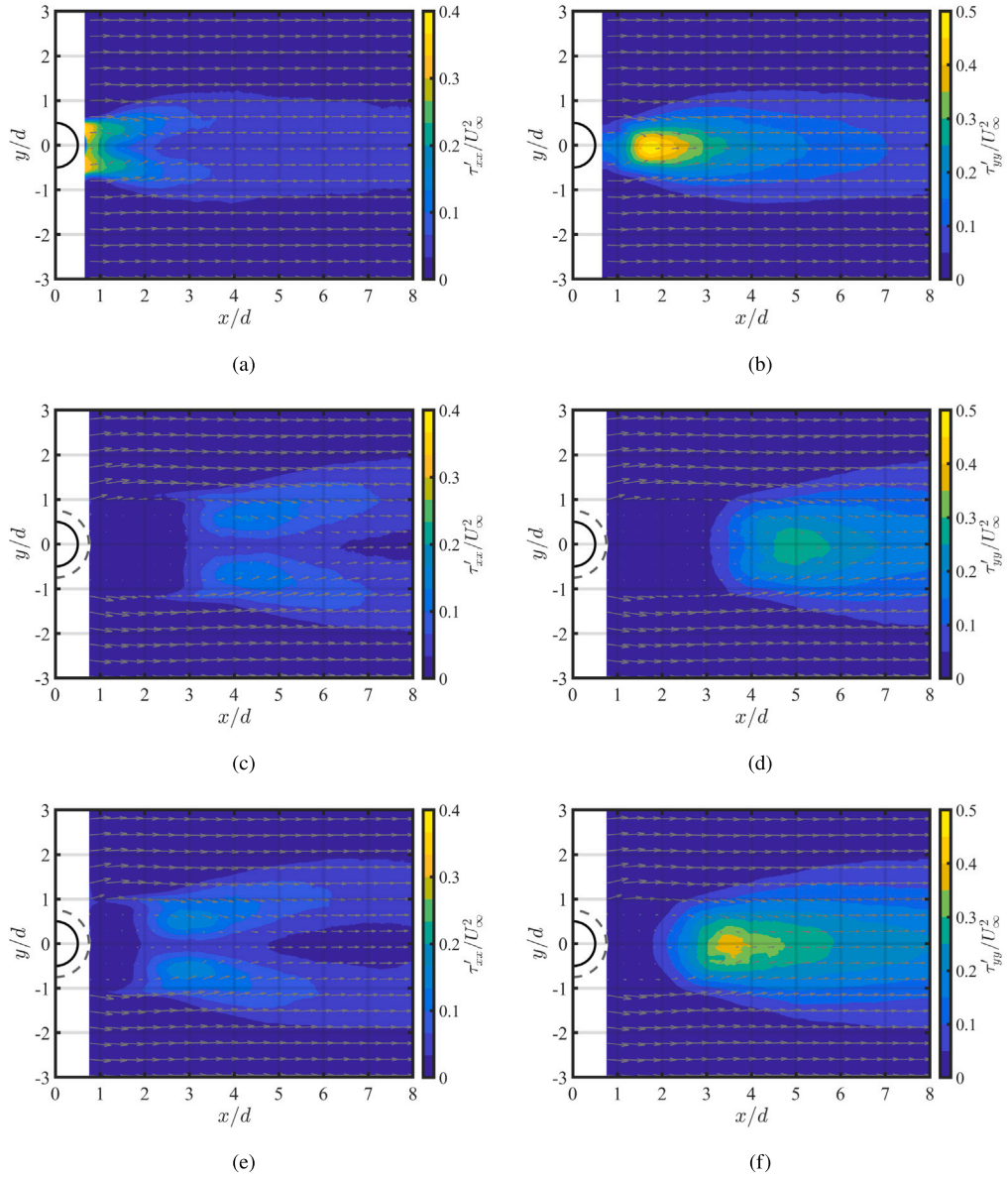
Fig. 17. Normalised flow statistics for the (a, b) bare cylinder and the cylinders coated with the (c, d) 30 PPI and (e, f) 10 PPI metal foams measured at Re_d = 6.8 \times 10^4 : (a, c, e) component \tau'_{xx} of the Reynolds stress tensor; (b, d, f) component \tau'_{yy} of the Reynolds stress tensor. The mean-flow streamlines are also indicated in the plot.
