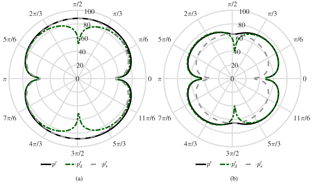
Fig. 24. Directivity patterns of the total, direct, and scattered acoustic pressure radiated at the vortex-shedding frequency by (a) the baseline and (b) the cylinder coated with the 30 PPI metal foam at Re_d = 6.8 \times 10^4 at a distance of r = 50d . The L_p values are expressed in dB with p_{ref} = 20 \mu\text{Pa} .
