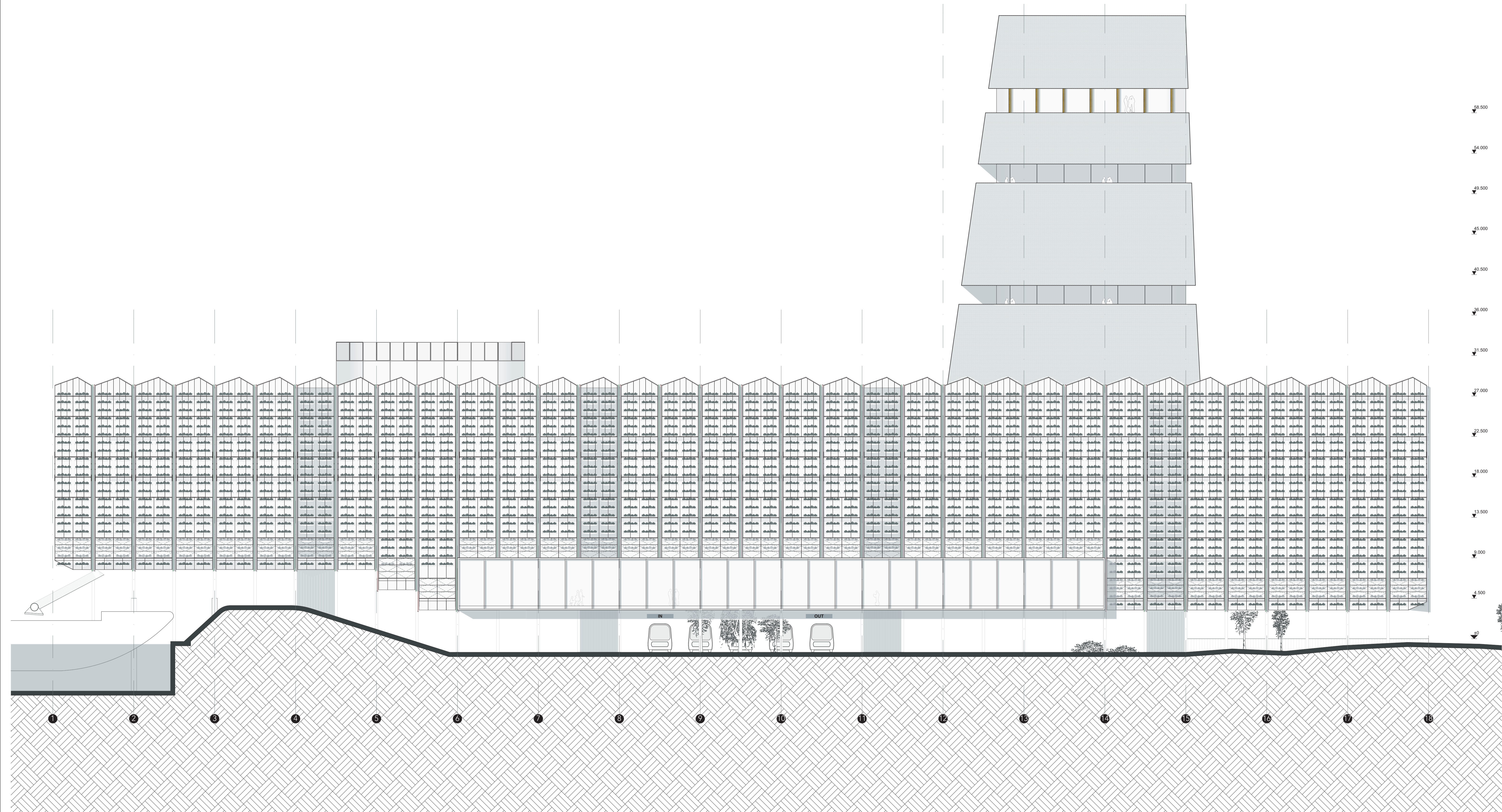
EAST FACADE MAIN FACTORY FACADE & LOADING DOCKS
