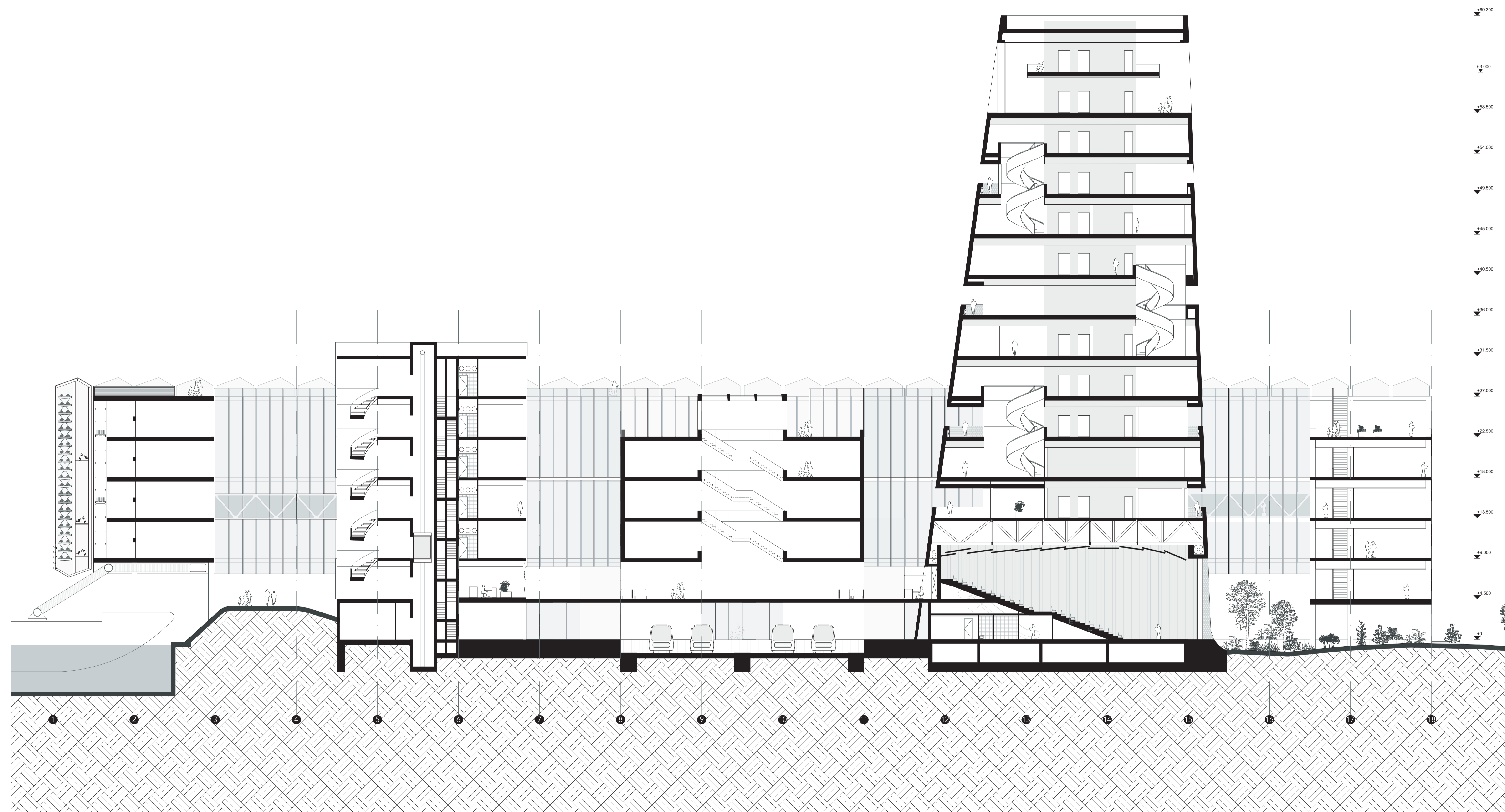
LONG SECTION SECTION AA
