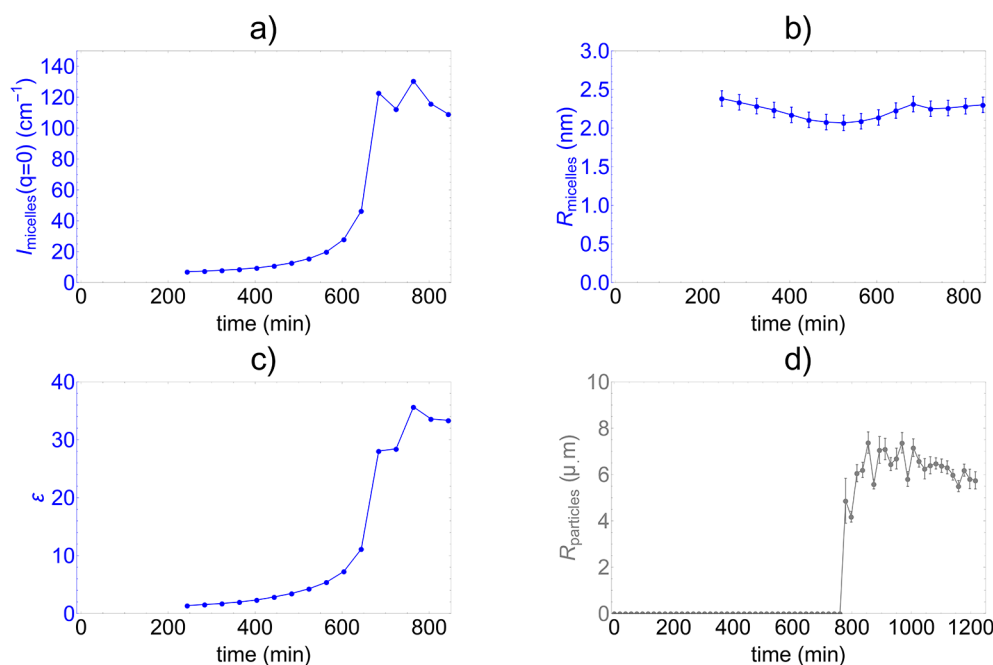
Figure 7. (a–c) Evolution with time of (a) I_{\text{micelles}}(q=0) ( \text{cm}^{-1} ), (b) the micelle radius R_{\text{micelles}} (nm), and (c) the ellipticity of the micelles \varepsilon extracted from the fitting of the SANS data measured previously at LOQ. Around 650 min, a sudden increase in scale and ellipticity is observed, associated with the formation of a gel. (d) Particle radius measured in SESANS (Delft) over time. At 800 min, a signal of very large particles is observed and corresponds to macroscopic phase separation.
