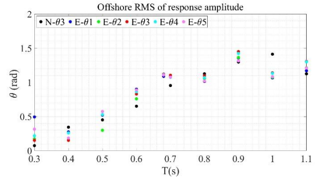
Figure 2: COMPARISON OF NUMERICAL (N \theta ) AND EXPERIMENTAL RESULTS (E \theta ) TO WAVE WITH SAME HEIGHT 0.05 m AND DIFFERENT PERIOD IN THE RANGE OF [0.3, 1.1] s
