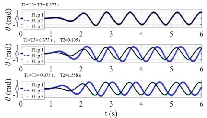
Figure 10: TIME-SERIES RESPONSES OF FLAPS IN AN ARRAY OF FIVE WITH DIFFERENT DYNAMIC CHARACTERISITCS
