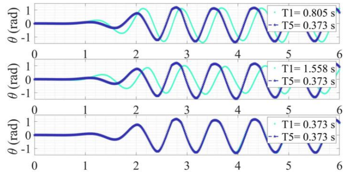
Figure 9: TIME-SERIES RESPONSES OF FLAPS IN AN ARRAY OF TWO WITH DIFFERENT DYNAMIC CHARACTERISITCS AND MAXIMUM GAP
