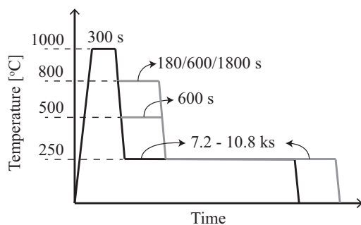
Fig. 1. Schematic of heat treatment profiles used for understanding the effect of grain-boundary cementite precipitation on bainite formation kinetics. The heating rate used during the heat treatments is 5 °C/s while the all cooling steps are carried out at −40 °C/s.
