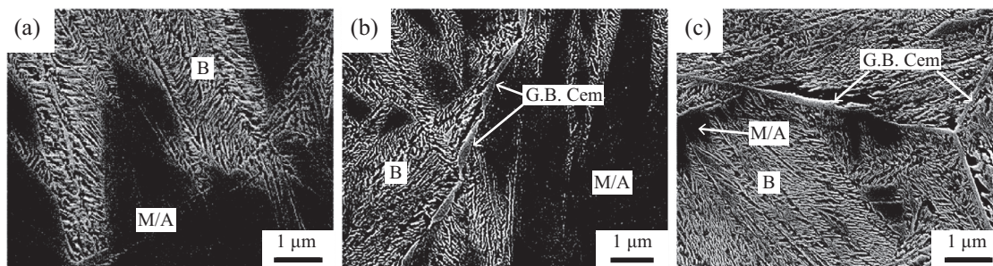
Fig. 3. SEM micrographs obtained after bainite formation treatment when it preceded by (a) no IAT (b) IAT at 500 °C for 10 min and (c) IAT at 800 °C for 10 min. Microstructure studies revealed Bainite (B), Martensite/Retained austenite (M/A) islands and grain-boundary cementite (G.B. Cem) depending on the corresponding treatment route.
