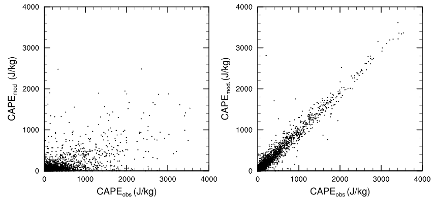
Figure 2. Scatterplot of (left) CAPE from soundings versus CAPE calculated for RACMO data and (right) CAPE supplemented with surface temperature and specific humidity from the sounding data.
