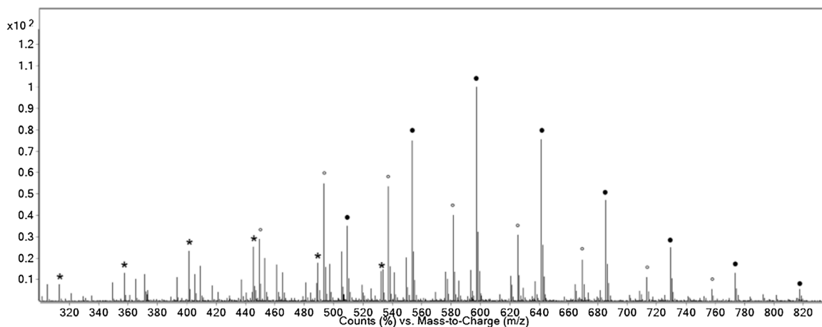
Fig. 2. Spectrum obtained from DESI-MS analysis of spots of lubricant from MSO condom, showing ion series corresponding to poly(ethylene glycol) decyl ether (*), octoxynol-9 [M + K]^+ (●) and [M + Na]^+ (°).
