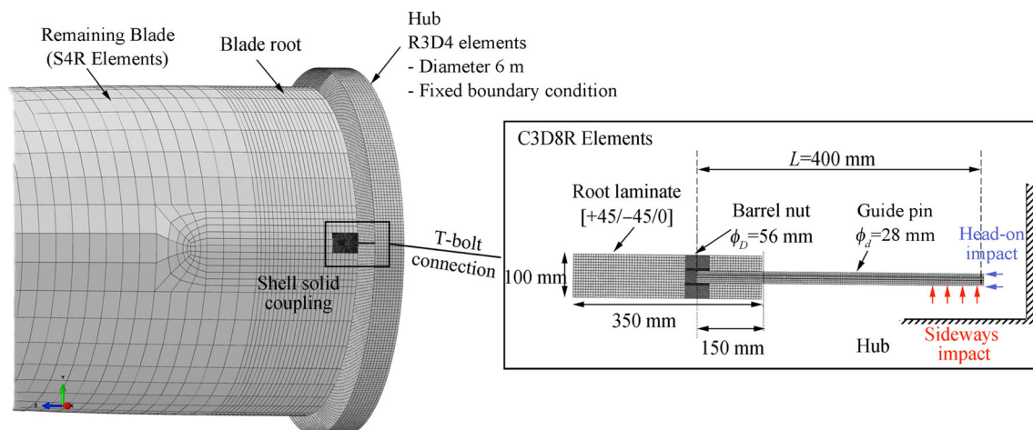
Figure 9 Finite element modelling of guide pin impact with hub for sideways and head-on impact scenarios
