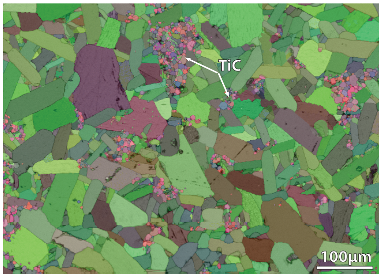
Figure 5.2: Microstructure of spark plasma sintered \text{Ti}_3\text{SiC}_2 from the starting composition of \text{Ti}:\text{Si}:\text{TiC} = 1:1:1.4 , with TiC content indicated.
