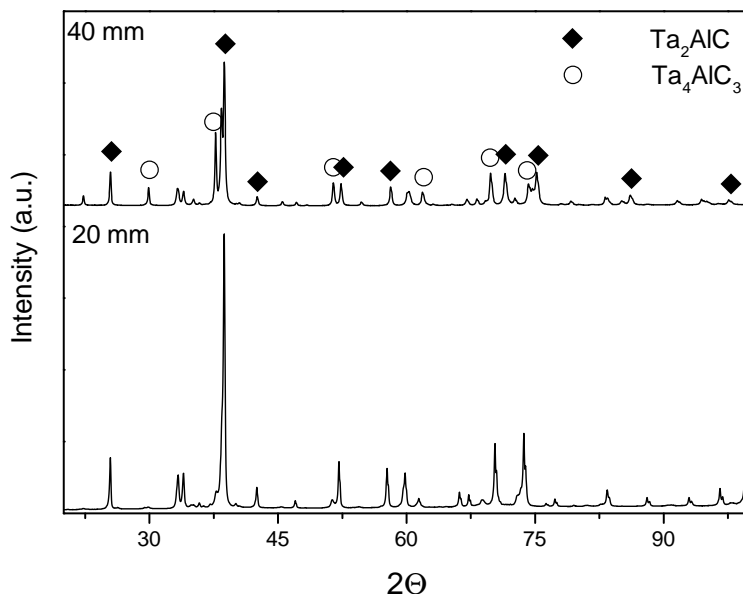
Figure 6.1: XRD patterns of spark plasma sintered Ta_2AlC with varying Ta_4AlC_3 content for two sample sizes.
