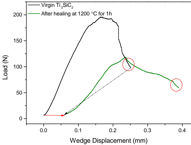
Figure 5.8: Load-Displacement curves of virgin and healed wedge loaded samples. The proposed unloading curve of the virgin sample is indicated (dashed black) and the second (green) curve was shifted to compensate for residual crack opening displacement (red arrow). The red circles show the identical material response for both materials for the final loading stages.
