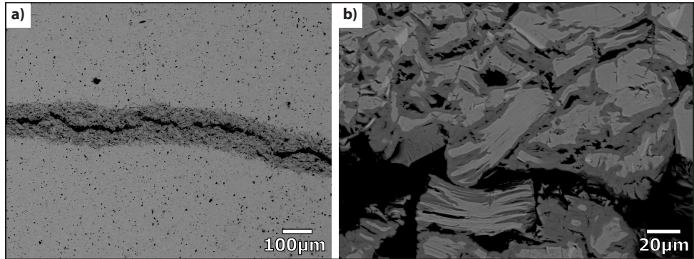
Figure 6.3: Backscattered electron image of Ta 2 AlC oxide after 16 h of oxidation at 600°C.
