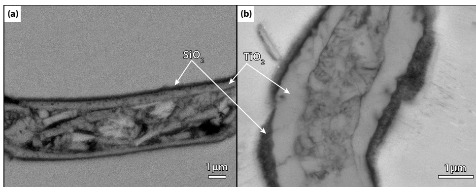
Figure 5.6: Crack in Ti_3SiC_2 (a) partially filled after oxidation at 1100\text{ }^\circ\text{C} for 1 h and (b) fully filled after oxidation at 1300\text{ }^\circ\text{C} for 1 h.
