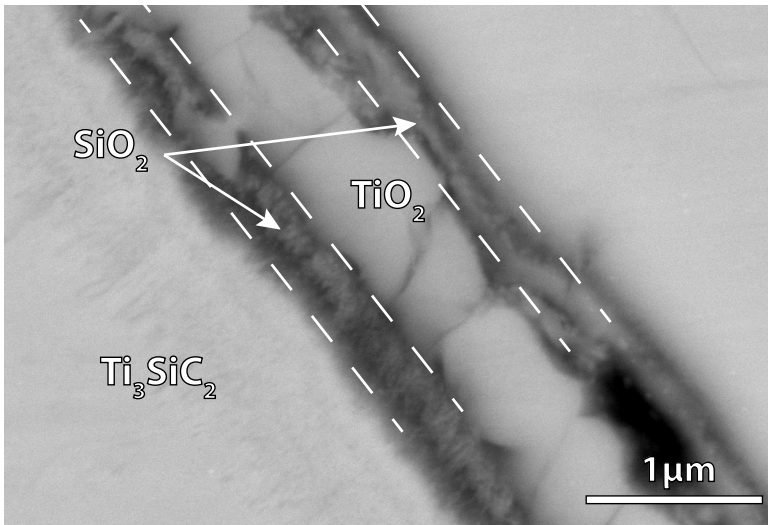
Figure 5.7: Crack in \text{Ti}_3\text{SiC}_2 after oxidation at 1300\text{ }^\circ\text{C} for 1 h. Local compositions as identified by SEM-XMA are indicated.
