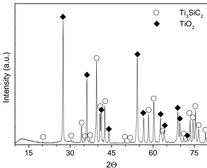
Figure 5.3: XRD pattern of \text{Ti}_3\text{SiC}_2 after oxidation at 1100\text{ }^\circ\text{C} for 20 h.
