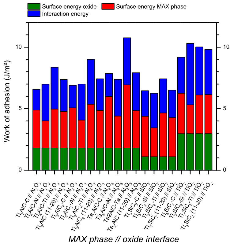
Figure 2.5: The work of adhesion for various MAX phases and their A-element oxide. The MAX phases with (0001) oriented surfaces terminate with C, M (=Ti, Ta) or A (=Al, Si) and are designated as M_{n+1}AX_n – terminating elements. The oxide surface orientation is (11-20), (111) and (110) for Al_2O_3 , SiO_2 and TiO_2 , respectively, and terminate with oxygen atoms (except TiO_2 which also has Ti atoms at its surface).
