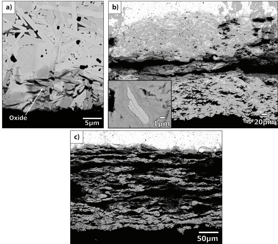
Figure 6.6: SEM images of oxide scales after 10 hours of isothermal oxidation of Ta 2 AlC in artificial air at a) 600, b) 700 and c) 800°C
