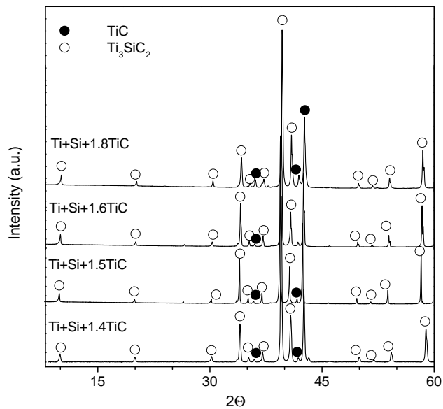
Figure 5.1: X-ray diffraction patterns for \text{Ti}_3\text{SiC}_2 spark plasma sintered from varying starting power molar ratios, viz.: Ti:Si:TIC = 1:1:X, with X equal to 1.4, 1.5, 1.6 and 1.8, respectively.
