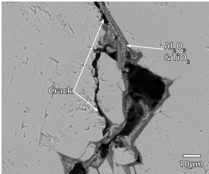
Figure 4.5: SEM backscattered electron image of cross-sectioned Ti_2AlC sample cracked 3 times with two intermediate healing treatments. The final induced crack runs through the previously formed TiO_2 and Al_2O_3 , as indicated.
