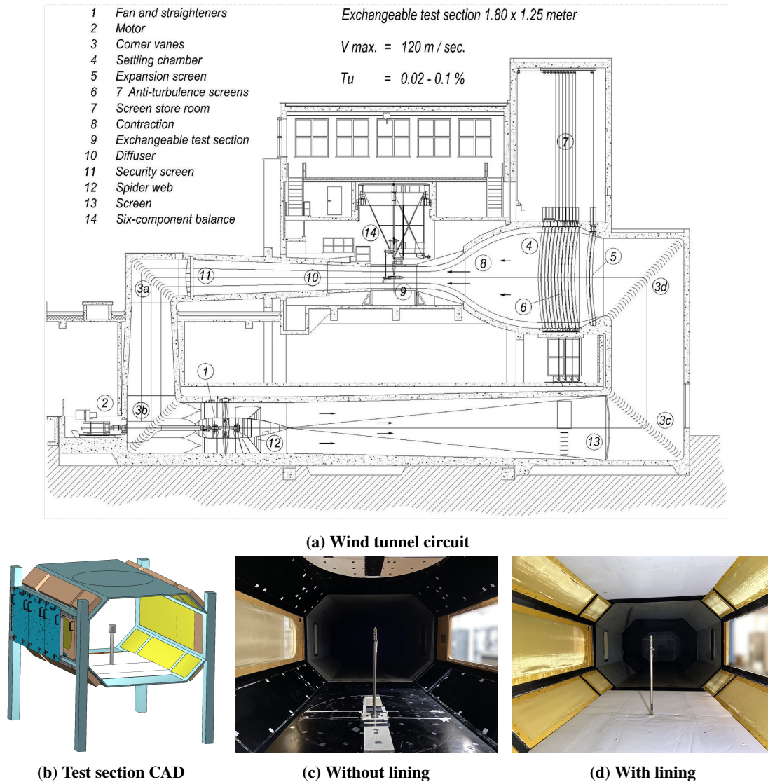
Fig. 1 Low turbulence tunnel circuit (top) [22], and aeroacoustic test section, as seen from the inlet: CAD of the test section (bottom-left), test section with baseline reflective walls (bottom-centre) and fully lined test section (bottom-right).
