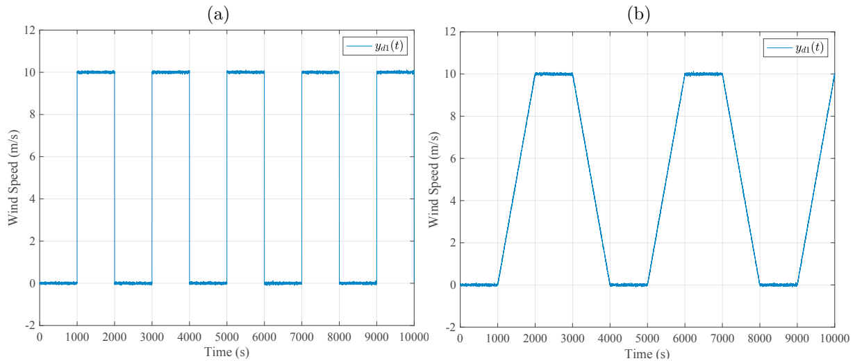
Fig. 2: Measured wind velocity y_{d1}(t) input signals: (a) Pulse function, (b) Ramp function
