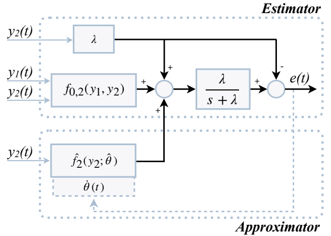
Fig. 1: Block diagram configuration of the EFOL scheme
