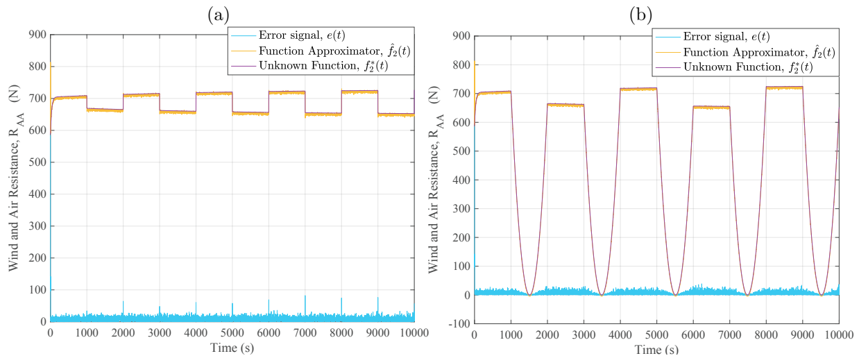
Fig. 3: Simulation results for: (a) Pulse y_{d1}(t) signal, (b) Ramp y_{d1}(t) signal
