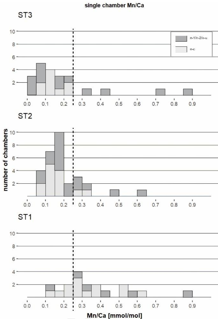
Figure 3. Histograms for all Mn/Ca measurements (individual chambers in dark grey, and central part of the test in light grey) for the three stations (bin width= 0.05 mmol/mol). Kruskal-Wallis test p value :< 0.001 (for data of n-1/n-2/n-u and n-c combined). Wilcoxon-Mann-Whitney post-hoc test p values: < 0.001 (ST1 vs ST2), < 0.001 (ST1 vs ST3) and 0.220 (ST2 vs ST3). Dashed line indicating 0.25 mmol/mol (see section 3 for explanation).
