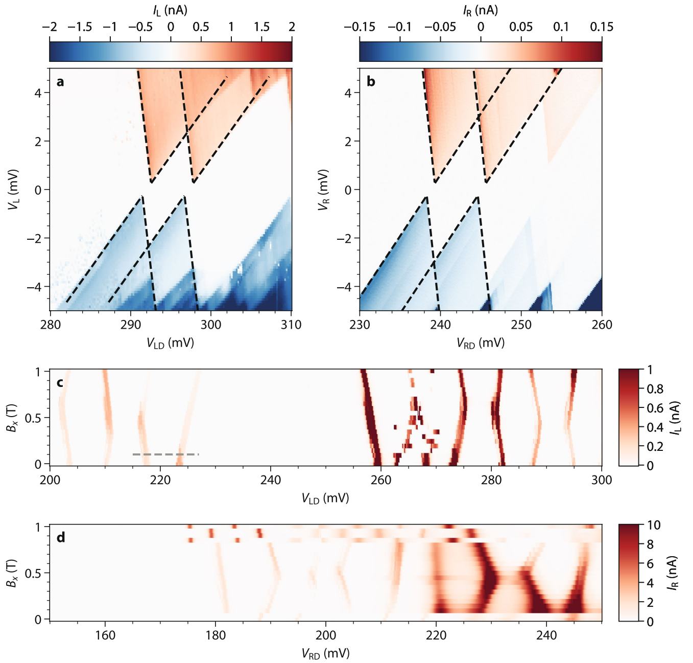
Extended Data Fig. 1 | QD characterization in device A. a , Coulomb blockade diamonds of the left QD. Superimposed dashed lines represent a model with charging energy 2.1 \text{ meV} , \Delta = 250 \mu\text{V} and lever arm 0.4 . V_{LD} shown here is different from other measurements of this resonance due to a drift in one tunnel barrier gate during the process of the experiment. b , Coulomb blockade diamonds of the right QD. Superimposed dashed lines represent a model with charging energy 2.75 \text{ meV} , \Delta = 250 \mu\text{V} and lever arm 0.435 . In both QDs, no subgap current is visible, indicating QDs are weakly coupled to S and retain their charge states. c , Current through the left QD at V_L = 500 \mu\text{V} measured
