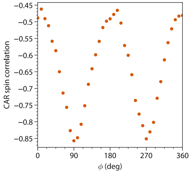
Extended Data Fig. 8 | Spin correlation analysis of the data in Fig. 4g. We define \text{CAR}^{\uparrow\uparrow} \equiv \langle |I_{\text{corr}}| \rangle for the \uparrow\uparrow spin configuration and similarly for the others, as defined in Fig. 4g. The spin correlation for a given B direction is calculated as (\text{CAR}^{\uparrow\uparrow} + \text{CAR}^{\downarrow\downarrow} - \text{CAR}^{\uparrow\downarrow} - \text{CAR}^{\downarrow\uparrow}) / (\text{CAR}^{\uparrow\uparrow} + \text{CAR}^{\downarrow\downarrow} + \text{CAR}^{\uparrow\downarrow} + \text{CAR}^{\downarrow\uparrow}) . Perfectly singlet pairing yields -1 spin correlation. The -0.86 correlation when B \parallel B_{\text{SO}} is limited by the measurement noise level and can be improved by more signal averaging or more sophisticated analysis methods that are less sensitive to noise. When B points along other directions, the spin anti-correlation reduces as expected for non-singlet pairing.
