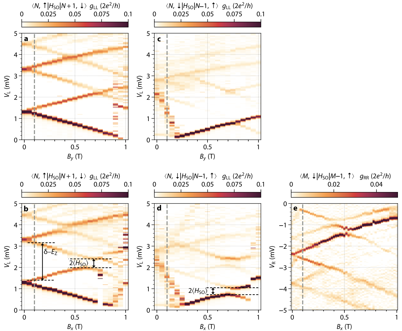
Extended Data Fig. 3 | QD excitation spectra measured using methods previously described 53 , from which we extract QD g -factor, level spacing and SOC. a, b , Left QD excitation spectra evolving under B applied along y ( a ) and x ( b ) for the spin-up ground state. Grey lines mark the field value at which the data in the main text are taken. The observation that opposite-spin excited states cross each other in a means spin is conserved, implying B_{SO} in the QD and B point along the same direction, that is, y . Opposite-spin states in b , by contrast, anti-cross due to SOC. The quantities needed to calculate the opposite-spin admixture weight (level spacing \delta , Zeeman splitting E_z and spin-orbit level repulsion gap 2\langle H_{SO} \rangle ) can be directly read from b (see Supplementary Information for details). b shows the largest value of spin-orbit level repulsion that we have measured in the QDs, which is used as an upper-bound estimation for the effect of SOC in QD in Supplementary Information. The Zeeman-splitting
