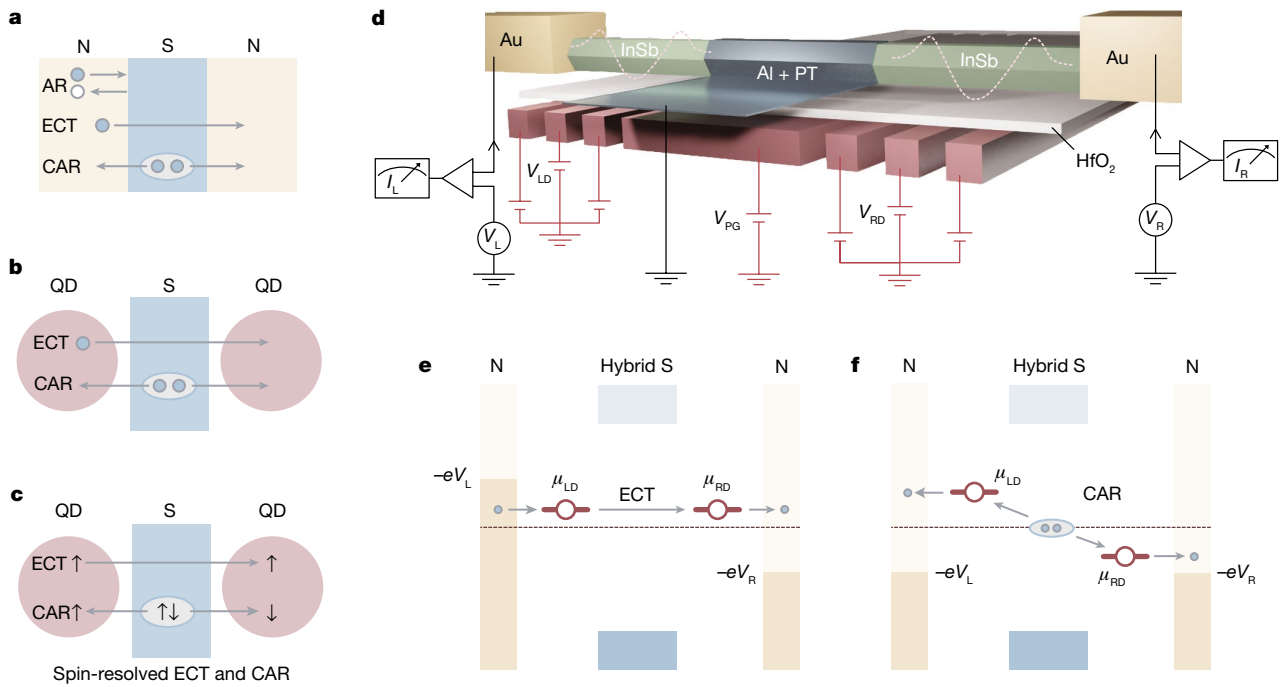
Fig. 1 | Transport processes, device and energy diagrams. a , Possible electron transport processes in a normal–superconductor–normal (N–S–N) structure: local Andreev reflection (AR), elastic co-tunnelling (ECT) and crossed Andreev reflection (CAR). b , A QD–S–QD structure enables only ECT and CAR. c , The QDs become spin-selective in a magnetic field, allowing us to distinguish ECT between equal spin states and CAR from a singlet Cooper pair involving
