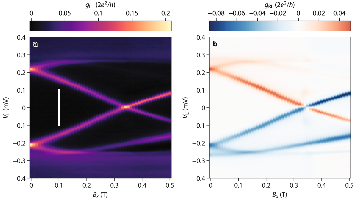
Extended Data Fig. 9 | B dependence of the energy spectrum in the middle hybrid segment of device A revealing a discrete Andreev bound state.
