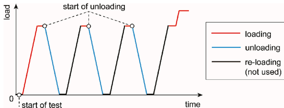
Fig. 8. A schematic cyclic loading history with one loading path and three unloading paths, to indicate the data organization during loading and unloading.
