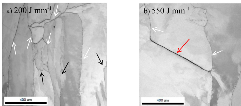
Fig. 14 – (A) and (b) shows the image quality maps of transverse sections in blocks A and E, respectively.
