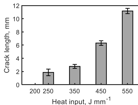
Fig. 10 – Experimentally derived variation of the crack length with the heat input. The average crack length per block is determined from observing four transverse sections taken at 35 mm, 40 mm, 45 mm and 50 mm from the starts of the deposits.
