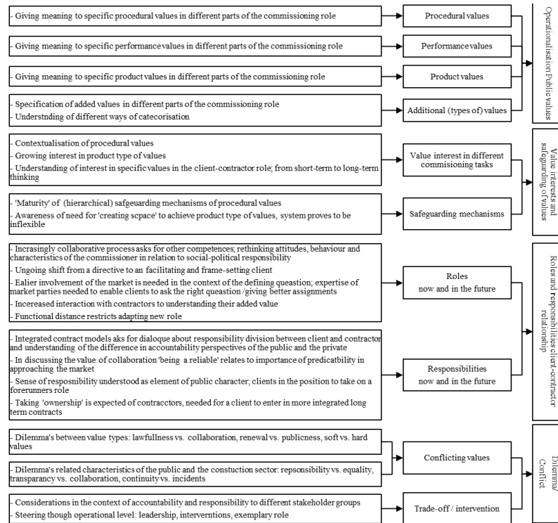
Figure 1: Data Structure
