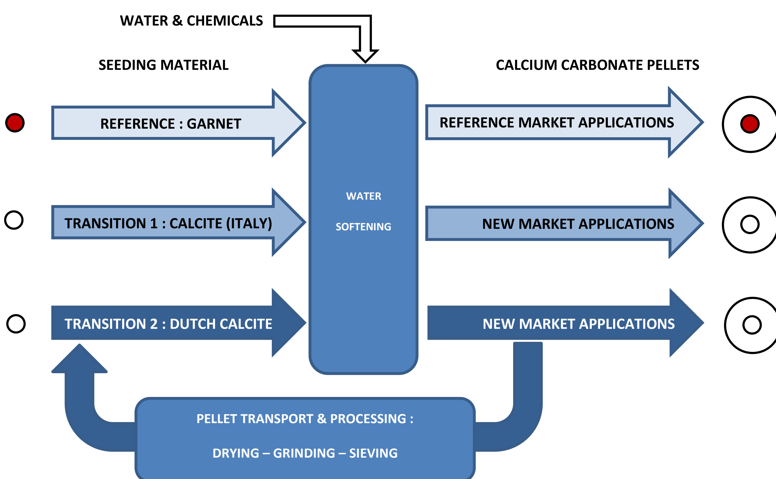
Figure 1 – Pellet softening by-product (calcium carbonate pellets) reuse concepts: reference case (garnet sand, Australia), 1st transition to high quality pellets (Italian calcite), and 2nd transition to Dutch calcite due to reuse of pellets as seeding material.
