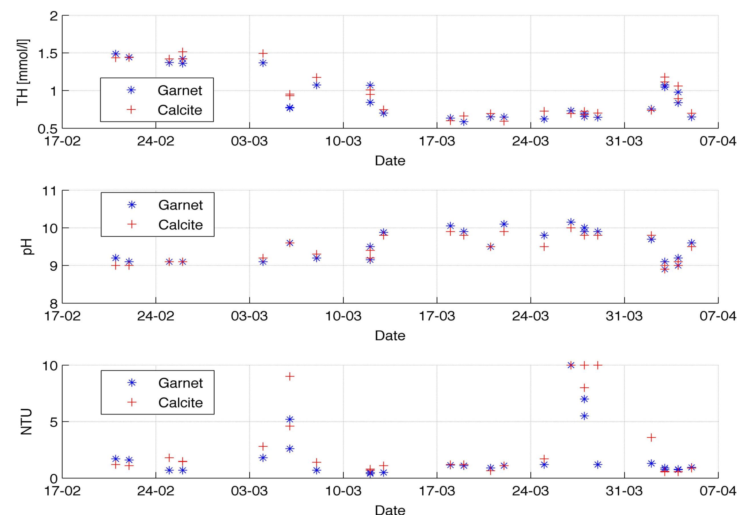
Figure 2 – Pilot plant research results: reactor effluent water quality for reference case (garnet) and reused calcite as seeding material
