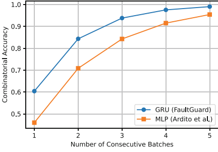
(a) Fault type prediction.
