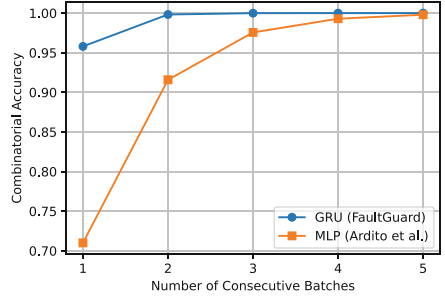
(b) Fault zone prediction.
