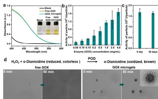
Figure 2. Local generation of H_2O_2 in the dual-functionalized crescent microgels. a , Absorbance spectra and color change (insert) of the solution without and with free GOX and dual-functionalized microgels in the gluconic acid-specific assay. 10 \mu g/mL free GOX, \sim 200 particles, 100 mM glucose, 100 mM hydroxylamine and 16 mM Fe^{3+} were used in this assay. b , Catalytic activity of the dual-functionalized microgels encapsulated with different concentrations of GOX. c , Stability of GOX in the dual-functionalized microgels after 30 days in PBS buffer solution. d , Visualization of the generation and distribution of H_2O_2 in the solution with free GOX (left) and dual-functionalized microgels (right, GOX=0.2 mg/mL) through oxidation reaction of o -dianisidine. These results are shown as the mean \pm s.d. of three independent experiments, with \sim 200 particles for each experiment. Scale bar 200 \mu m .
