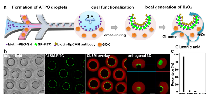
Figure 1. Fabrication of dual-functionalized crescent microgels. a , Schematic of the fabrication of dual-functionalized crescent microgels in a microfluidic device and their local generation of H_2O_2 based on the catalytic oxidation of glucose by GOX. b , Bright-field microscope image, confocal laser scanning microscope (CLSM) images of the dual-functionalized crescent microgels. Orthogonal images in x - y , x - z and y - z planes were shown, along with a 3D image. c , The distribution of streptavidin modification of \sim 200 microgels. The microgels were labelled by rhodamine B (red) and streptavidin were labelled by fluorescein isothiocyanate (FITC, green). Scale bar 50 \mu m .
