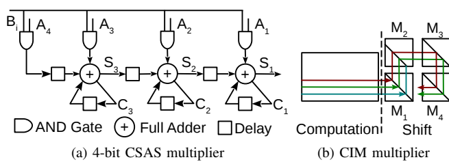
Fig. 3: CIM multiplier design.
