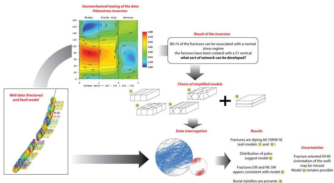
Figure 2: method of interpretation and simplification of fracture data coming from wellbore data. This workflow is intended to be used to produce geologically constrained training images to be integrated in the MPS-based workflow
