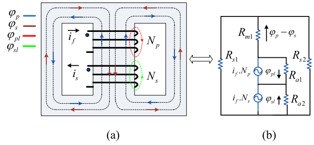
Fig. 9. a) Magnetic structure of SSSR b) electric equivalent circuit model.
