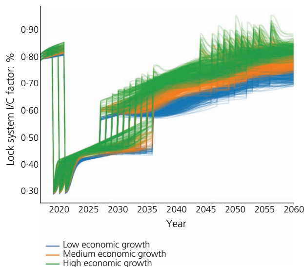
Figure 3. Lock system I/C factor divided by economic growth
