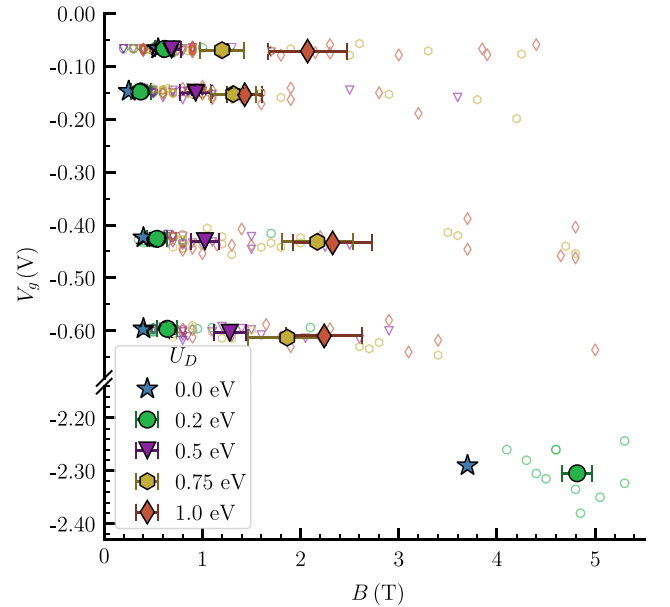
FIG. 16. Topological phase phase diagram in the presence of disorder. Plotted are the positions of the local minima B_c^* of critical magnetic fields in B, V_g plane. Empty dots corresponds to separate disorder realizations, filled symbols are disorder averages with the corresponding error bars. Increasing disorder strength leads to larger critical fields.
