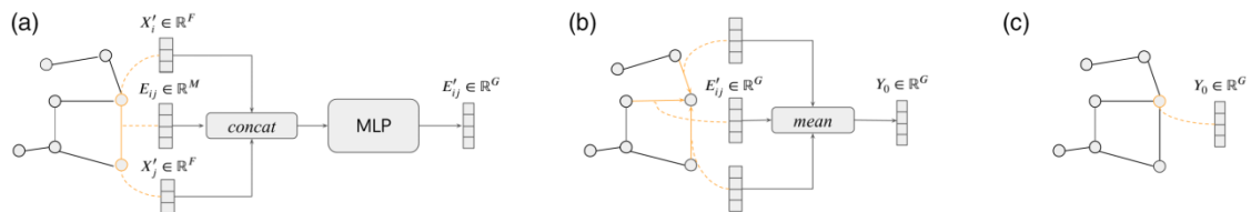
Figure 4 | Procedure to determine the node embeddings Y_0 . (a) The edge attributes E_{ij} and node attributes of the incident nodes X_i and X_j are concatenated and then fed to an MLP shared across all edges, to determine an edge embedding E'_{ij} . (b) For every node, the embeddings of incidental edges E'_{ij} are aggregated to determine the final node embedding Y_0 . (c) Node embeddings for every node are finally fed to the model.
