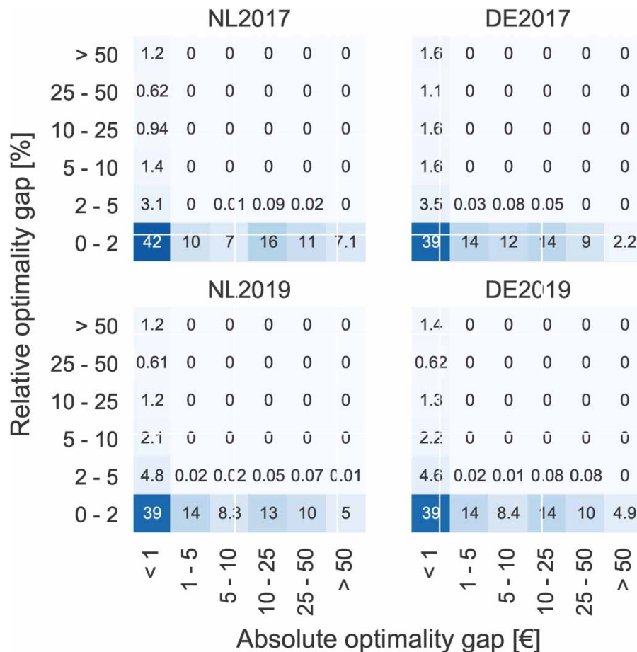
Figure 5 | Percentage of occurrence of the combined termination conditions for the individual optimisation problems. Gurobi termination settings are at an absolute optimality gap of €1, or at a relative optimality gap of 2%.
