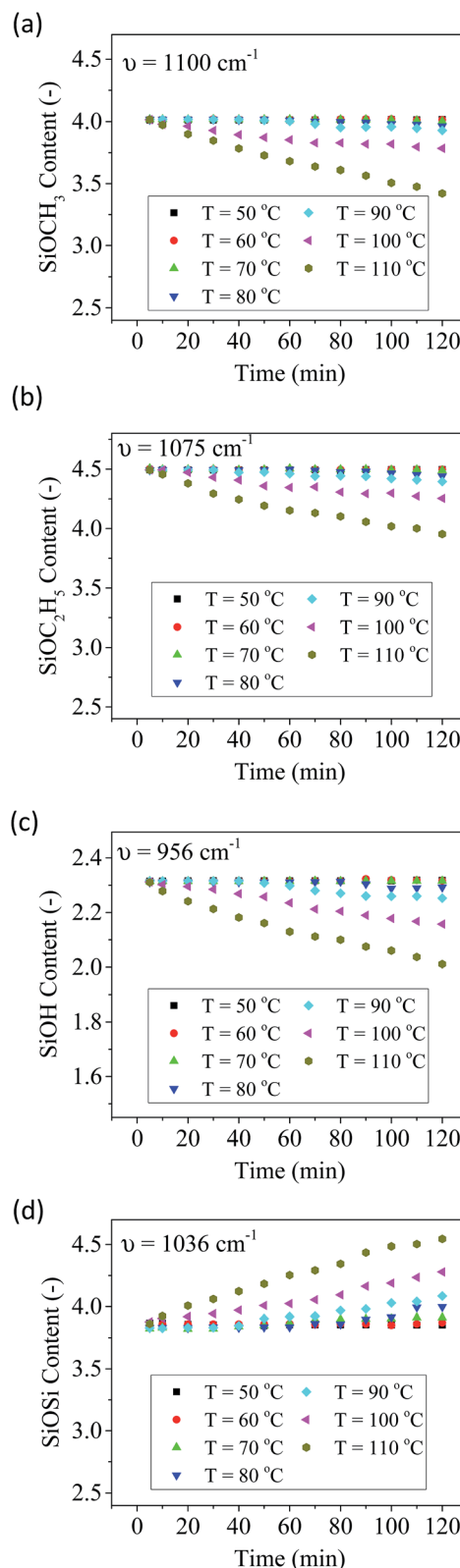
Fig. 4 Evolution of \text{SiOCH}_3 (a), \text{SiOC}_2\text{H}_5 (b), \text{SiOH} groups (c) and Si–O–Si bonds (d) of the hybrid sol–gel polymer cured for 2 h and further cured at different temperatures in a rheological time-sweep scan.
