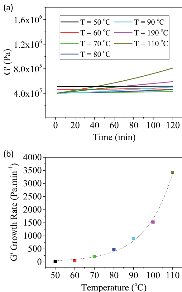
Fig. 2 Rheological time-sweep scans at 1 Hz and different temperatures (a) and the corresponding growth rate of the elastic modulus ( G' ) with temperature (b).
