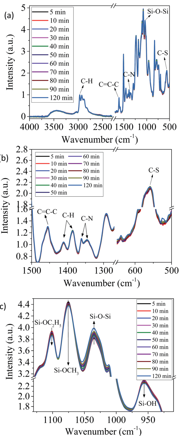
Fig. 3 FTIR spectra of the hybrid sol-gel polymer cured for 2 h and further cured at 100 °C during a time-sweep rheological scan: spectral range of 4000–500 \text{cm}^{-1} (a), 1500–500 \text{cm}^{-1} (b) and 1150–900 \text{cm}^{-1} (c).
